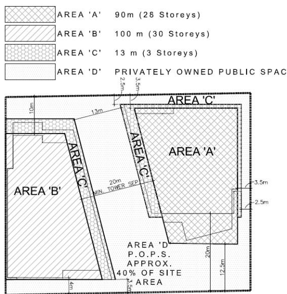
Figure 13: The plan illustrates the podium area, the towers setbacks and heights and separation from the lot lines. Source: Hobin Architecture 2020.
