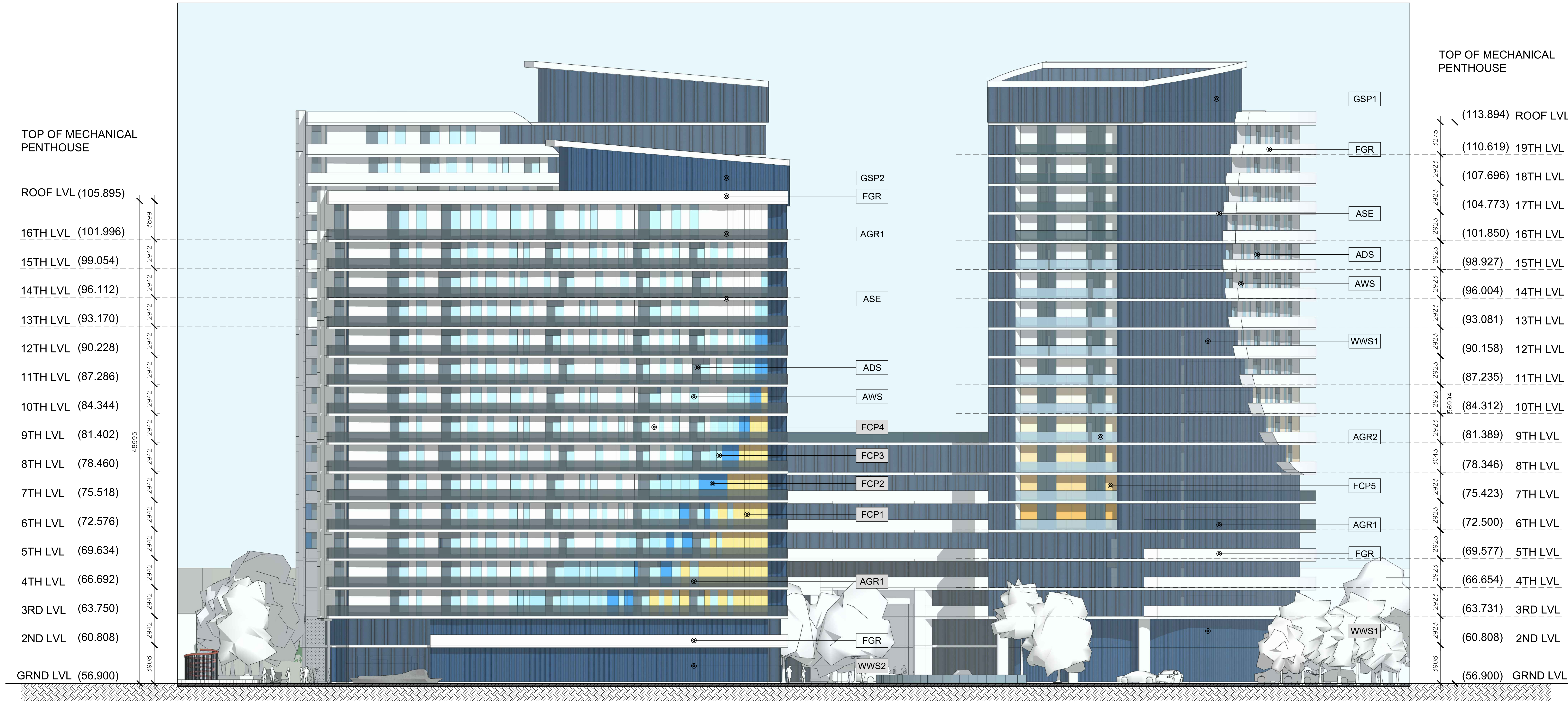
WEST ELEVATION SCALE 1:150 TOWER C & TOWER B
