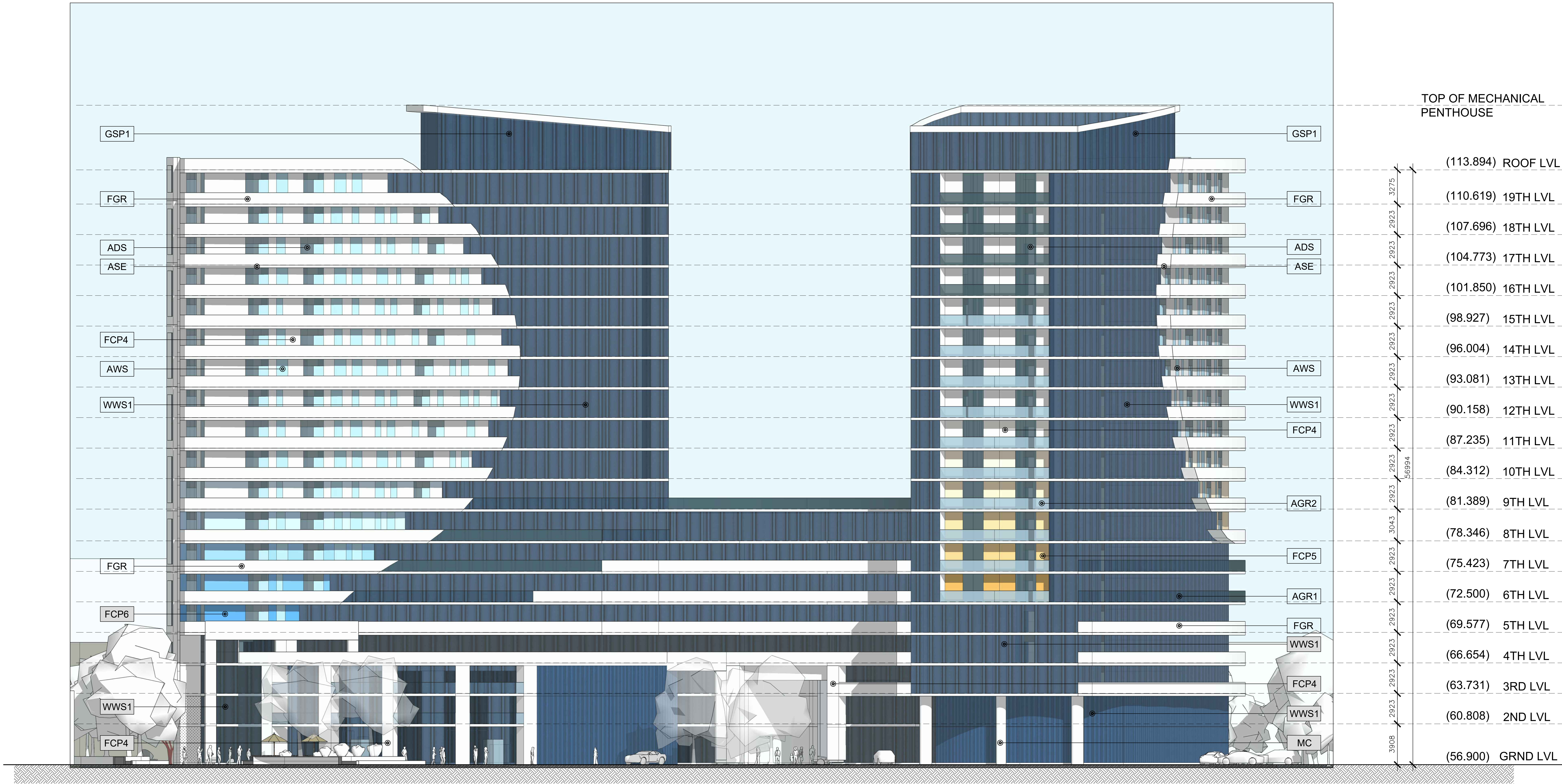
COURTYARD ELEVATION SCALE 1:150 TOWER A & TOWER B
