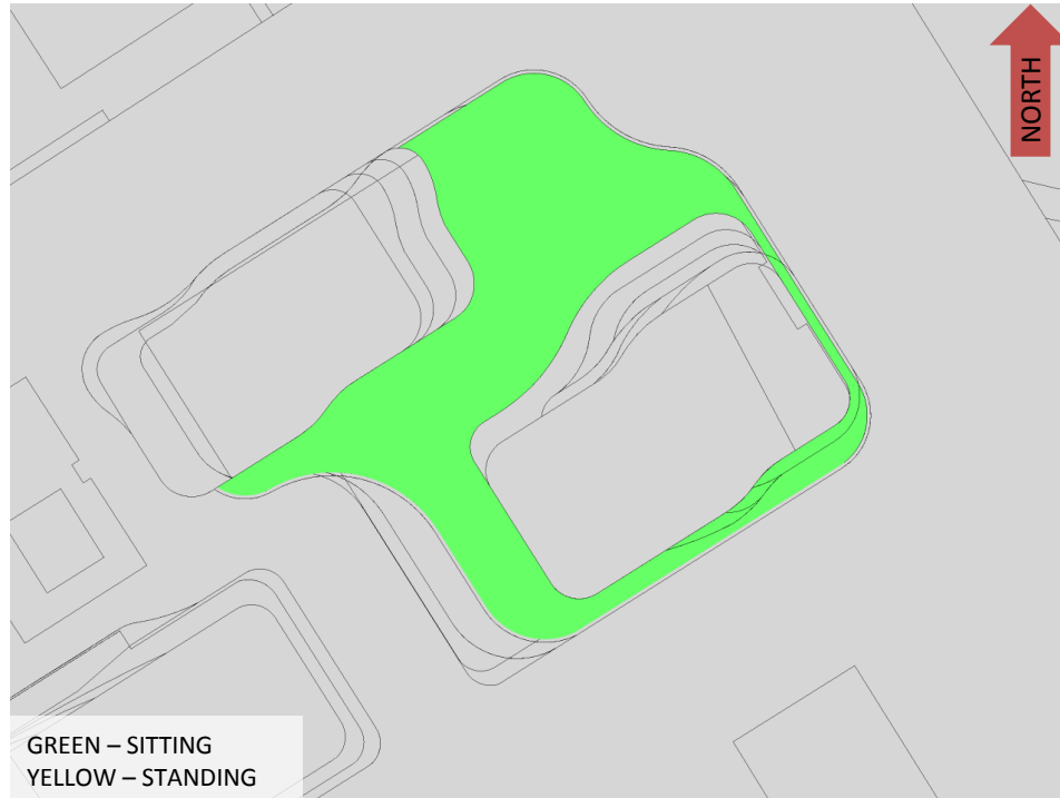
FIGURE 4B: SUMMER – OUTDOOR AMENITY AREA WIND CONDITIONS
