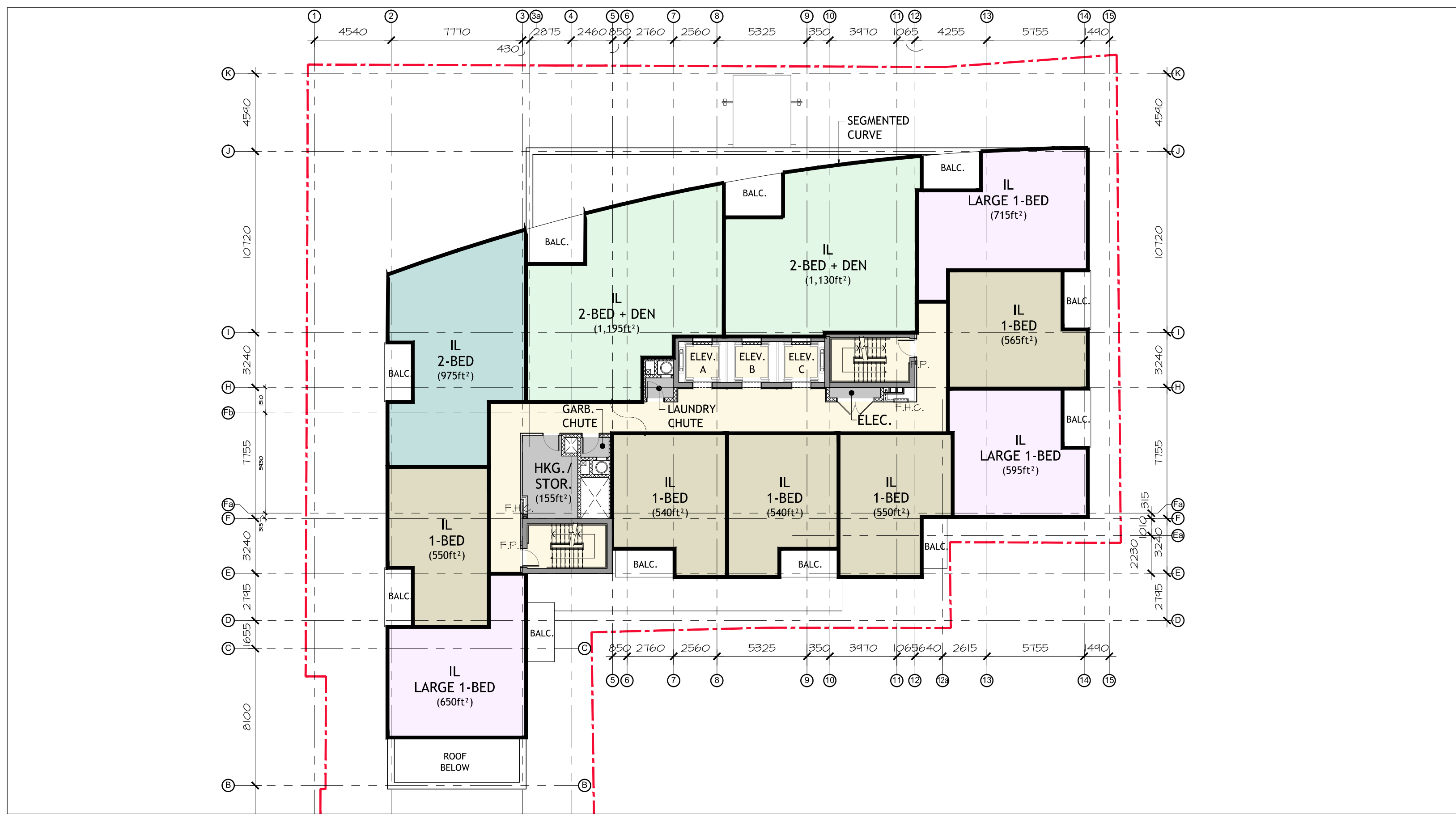
Proposed Levels 4-12 | Independent Living (IL)
