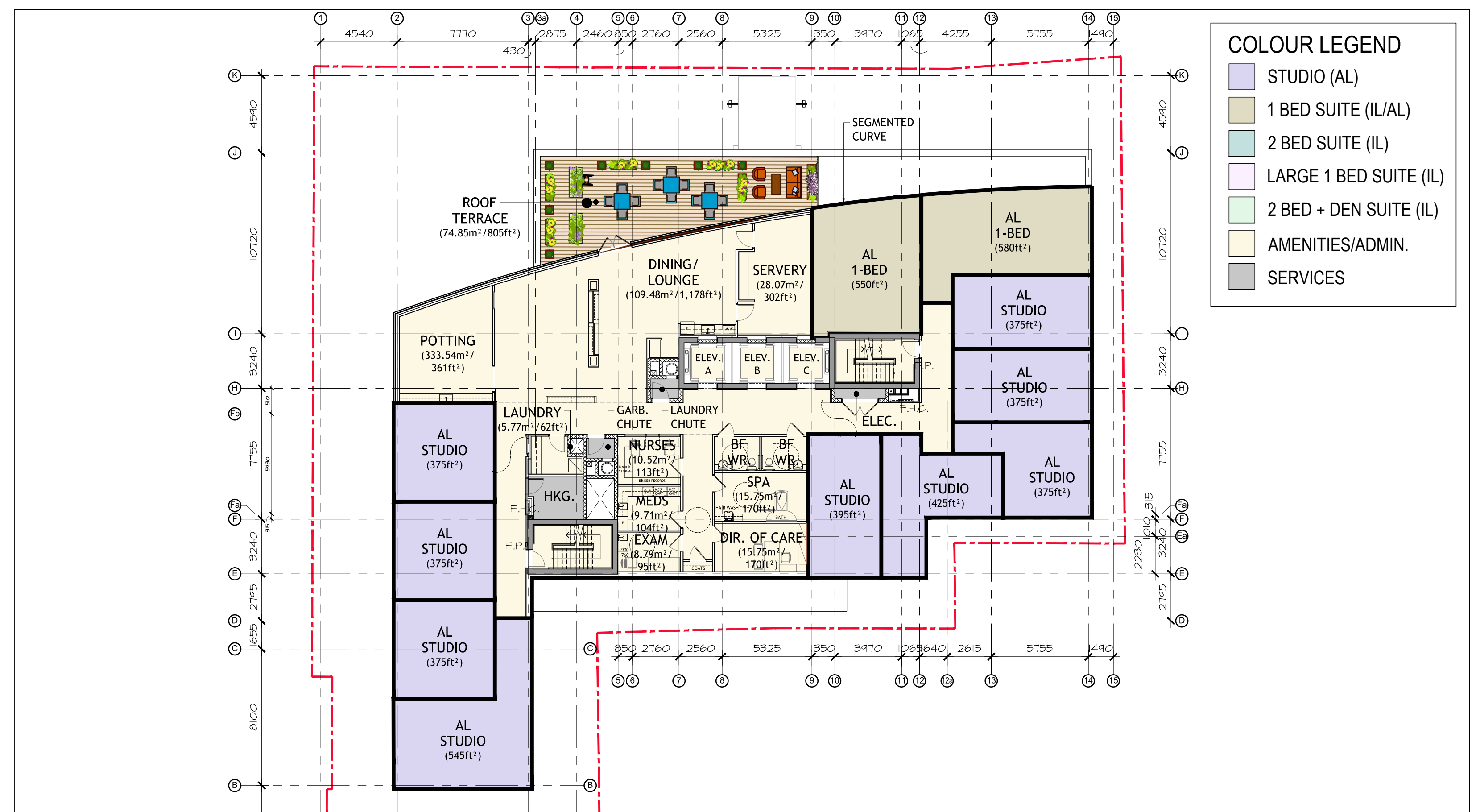
Proposed Level 3 | Assisted Living (AL)
