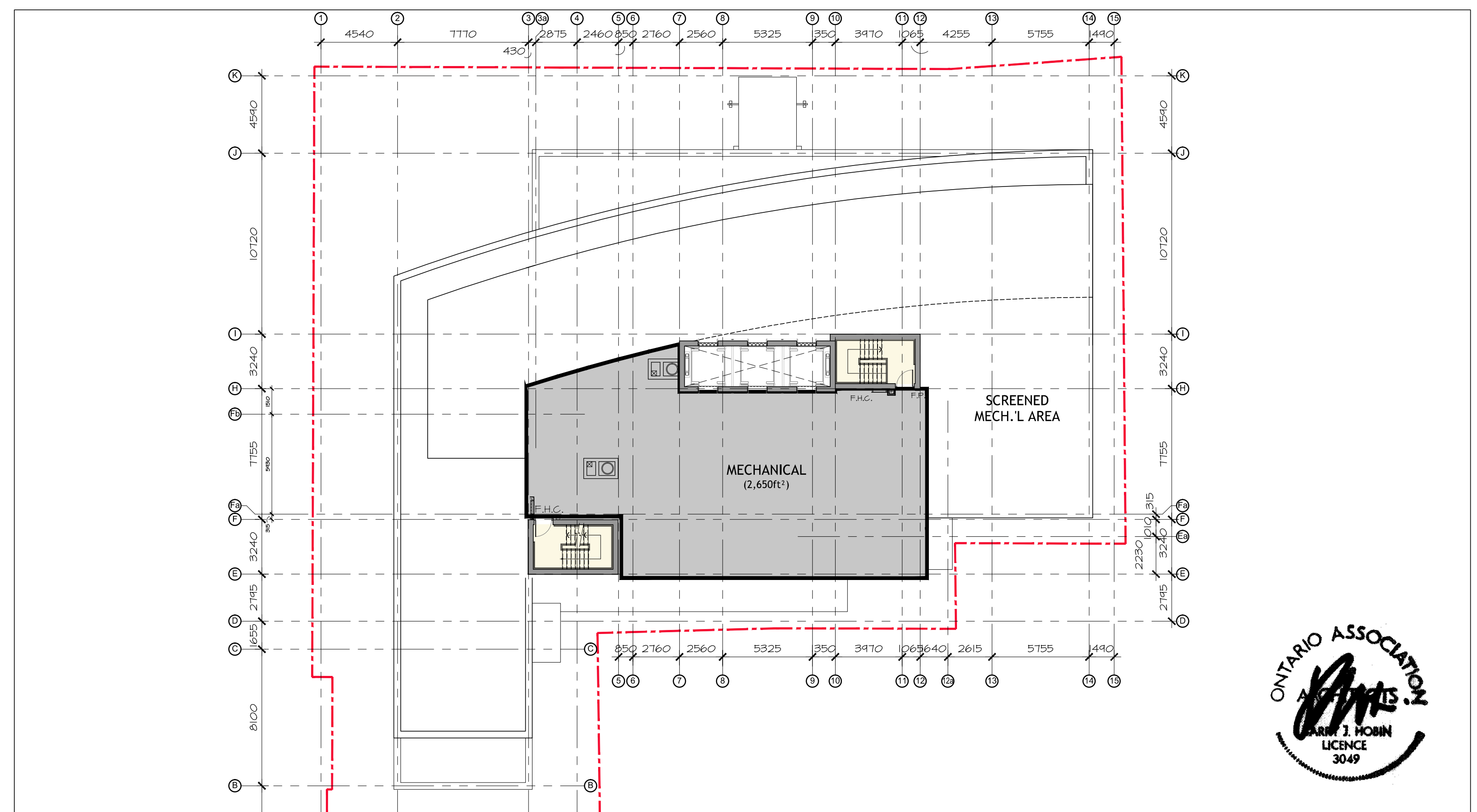
Proposed Mechanical Penthouse
