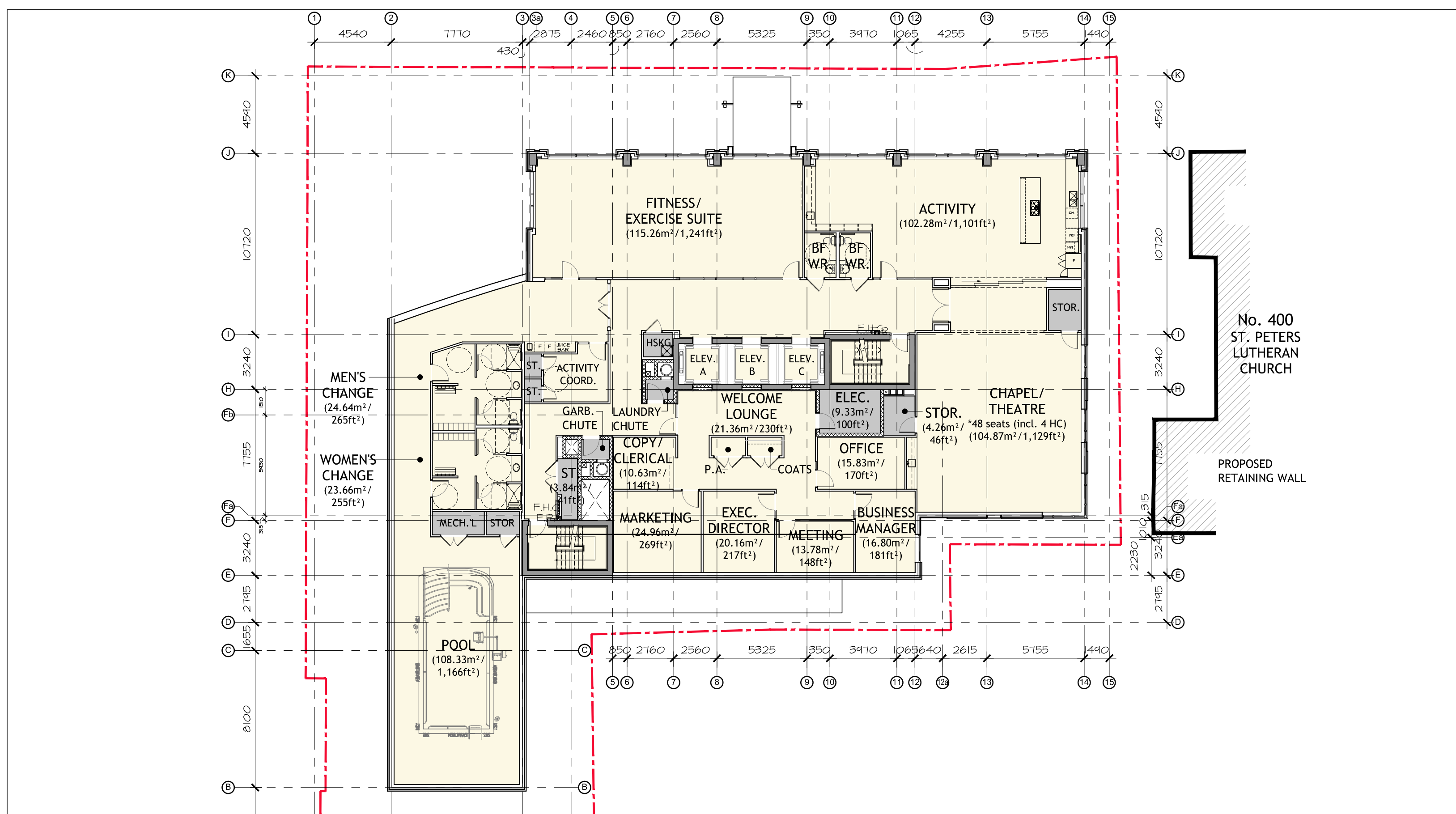
Proposed Level 2 | Amenities & Administration
