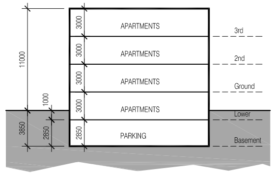
SECTION DIAGRAM
