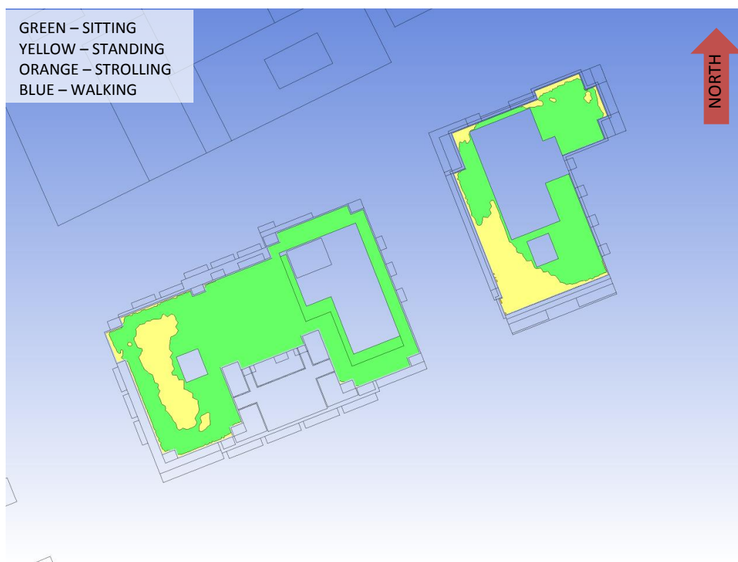
FIGURE 4B: SUMMER – LEVEL 16 OUTDOOR AMENITY AREA WIND CONDITIONS
