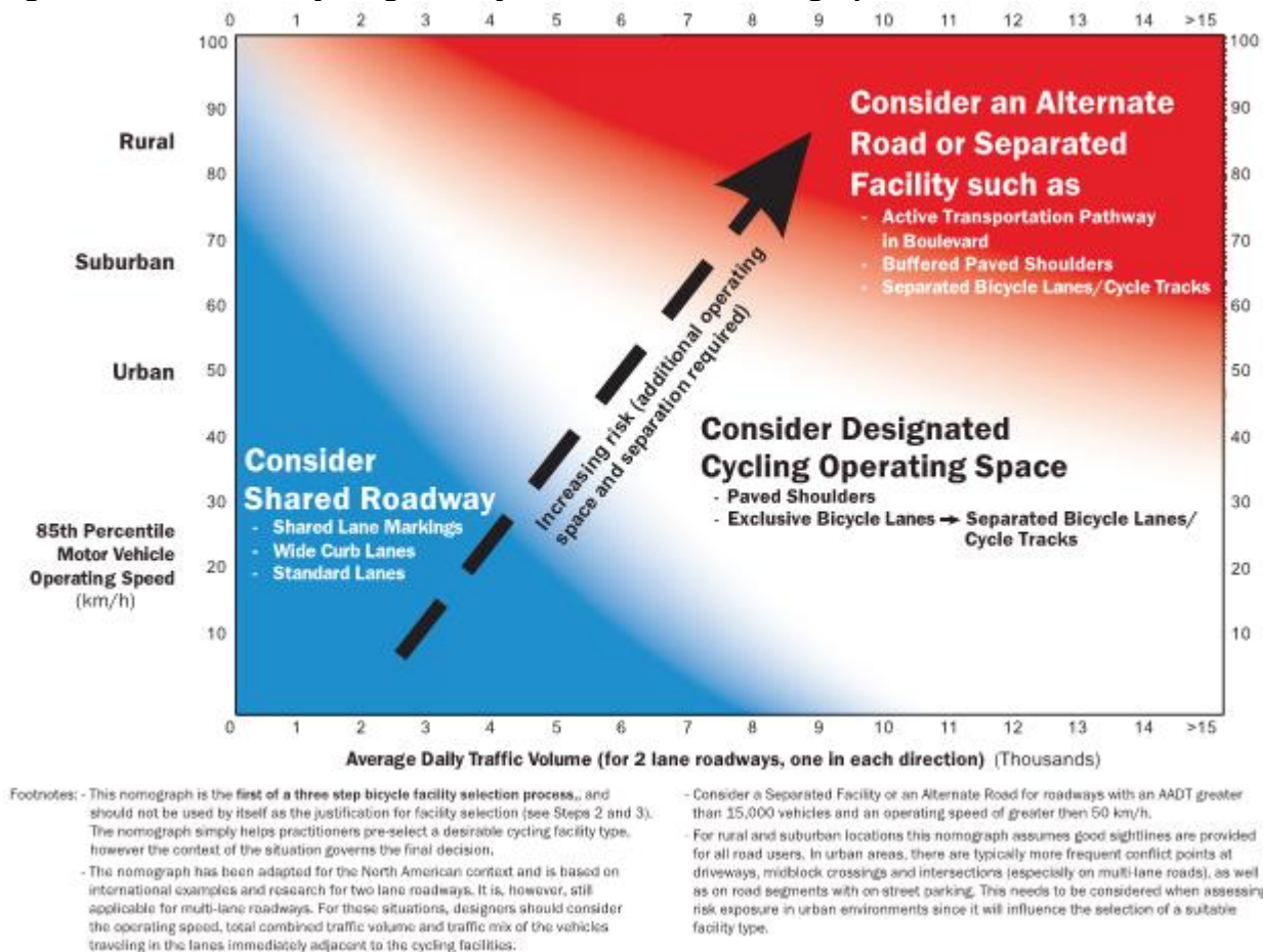
Figure 10: Desirable Cycling Facility Pre-Selection Nomograph
