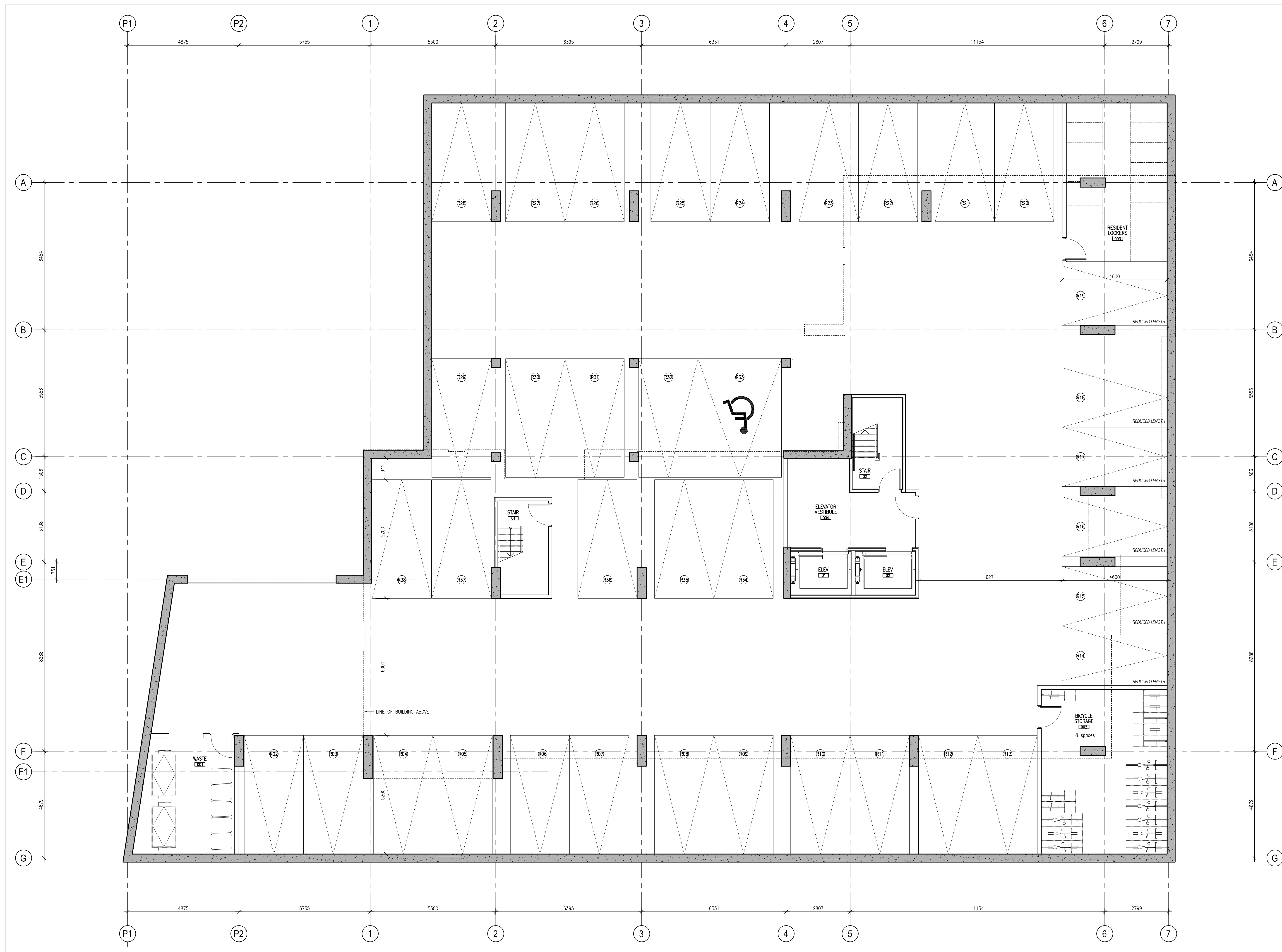
1 LEVEL P1 FLOOR PLAN A100 SCALE: 1:75
