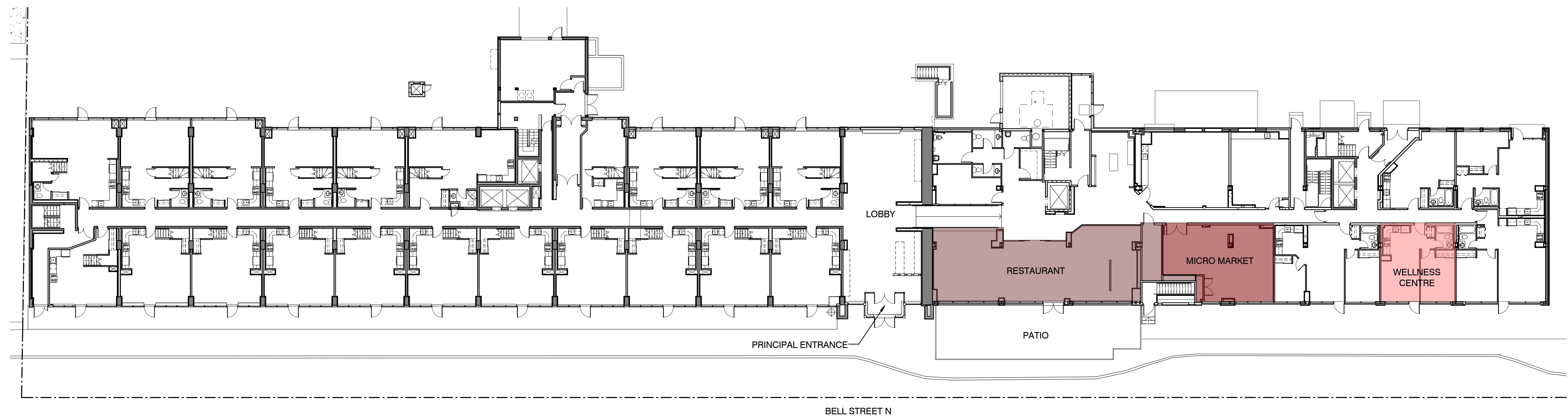
GROUND FLOOR PLAN SCALE: 1/16" = 1'-0" NOVEMBER 14, 2017
