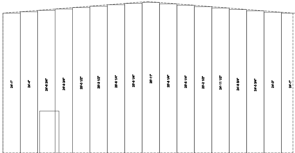
ENDWALL SHEETING & TRIM: FRAME LINE 4
