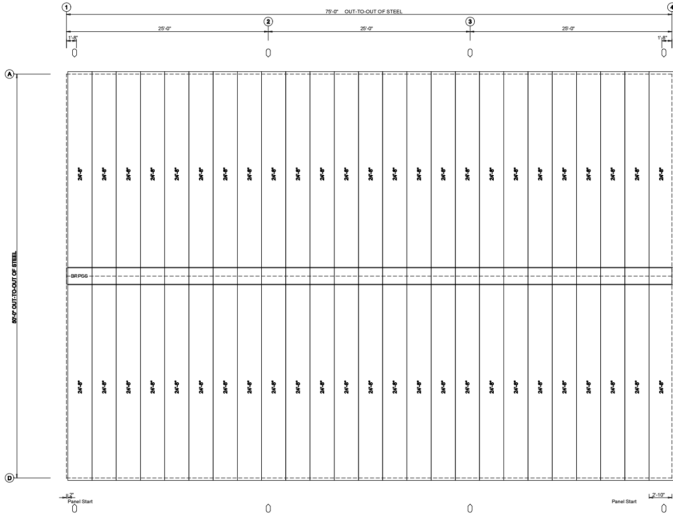
ROOF SHEETING PLAN
