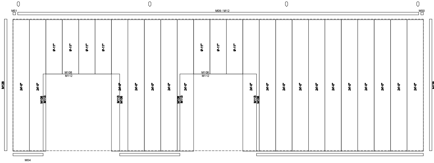
SIDEWALL SHEETING & TRIM: FRAME LINE D PANELS: 26 Ga. STORM SEAL - NRO - - PAINTED FINISH - STD
