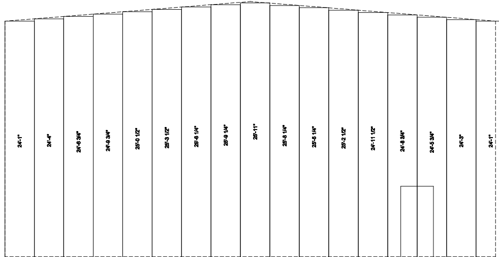
ENDWALL SHEETING & TRIM: FRAME LINE 1
