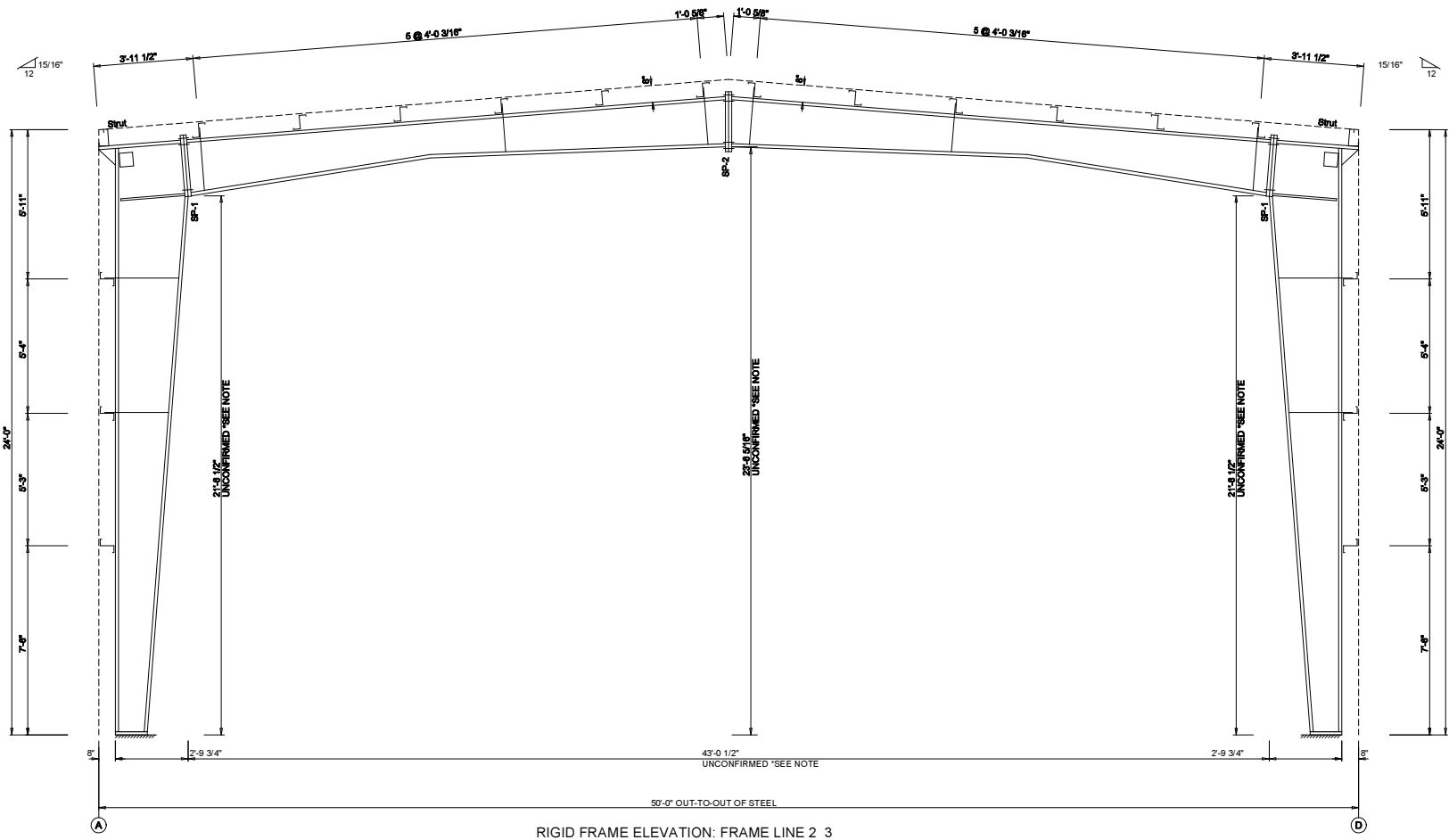
RIGID FRAME ELEVATION: FRAME LINE 2 3
