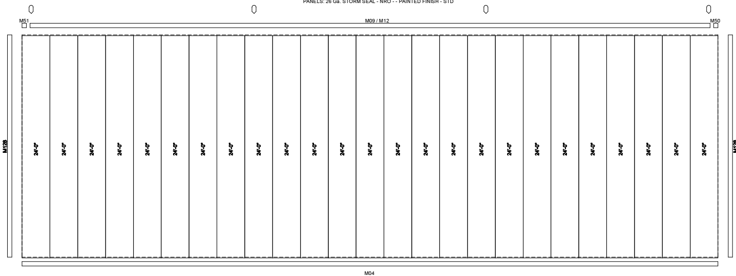
SIDEWALL SHEETING & TRIM: FRAME LINE A PANELS: 26 Ga. STORM SEAL - NRO - - PAINTED FINISH - STD
