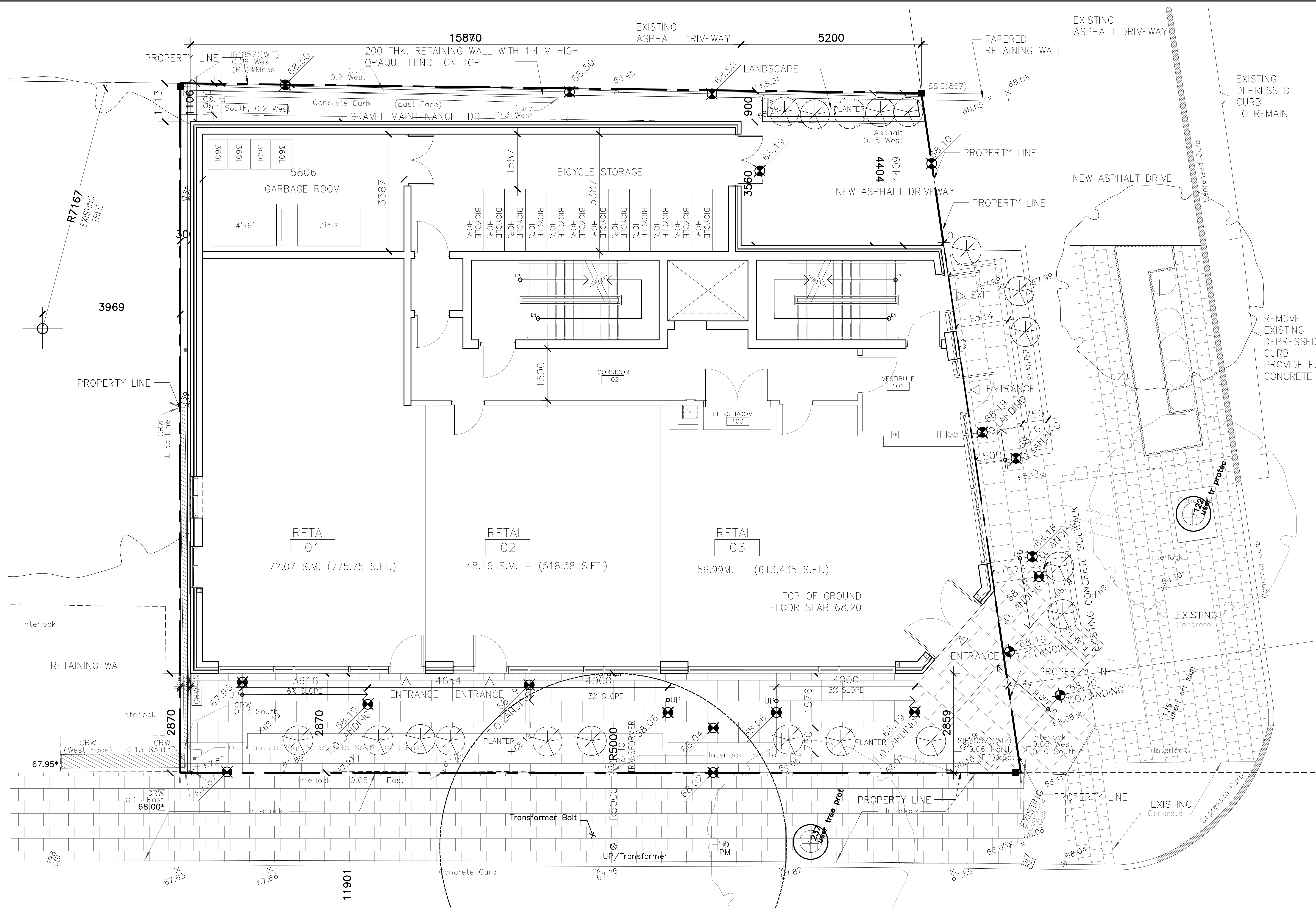
1 GROUND FLOOR PLAN SCALE 1:50 A1.1
