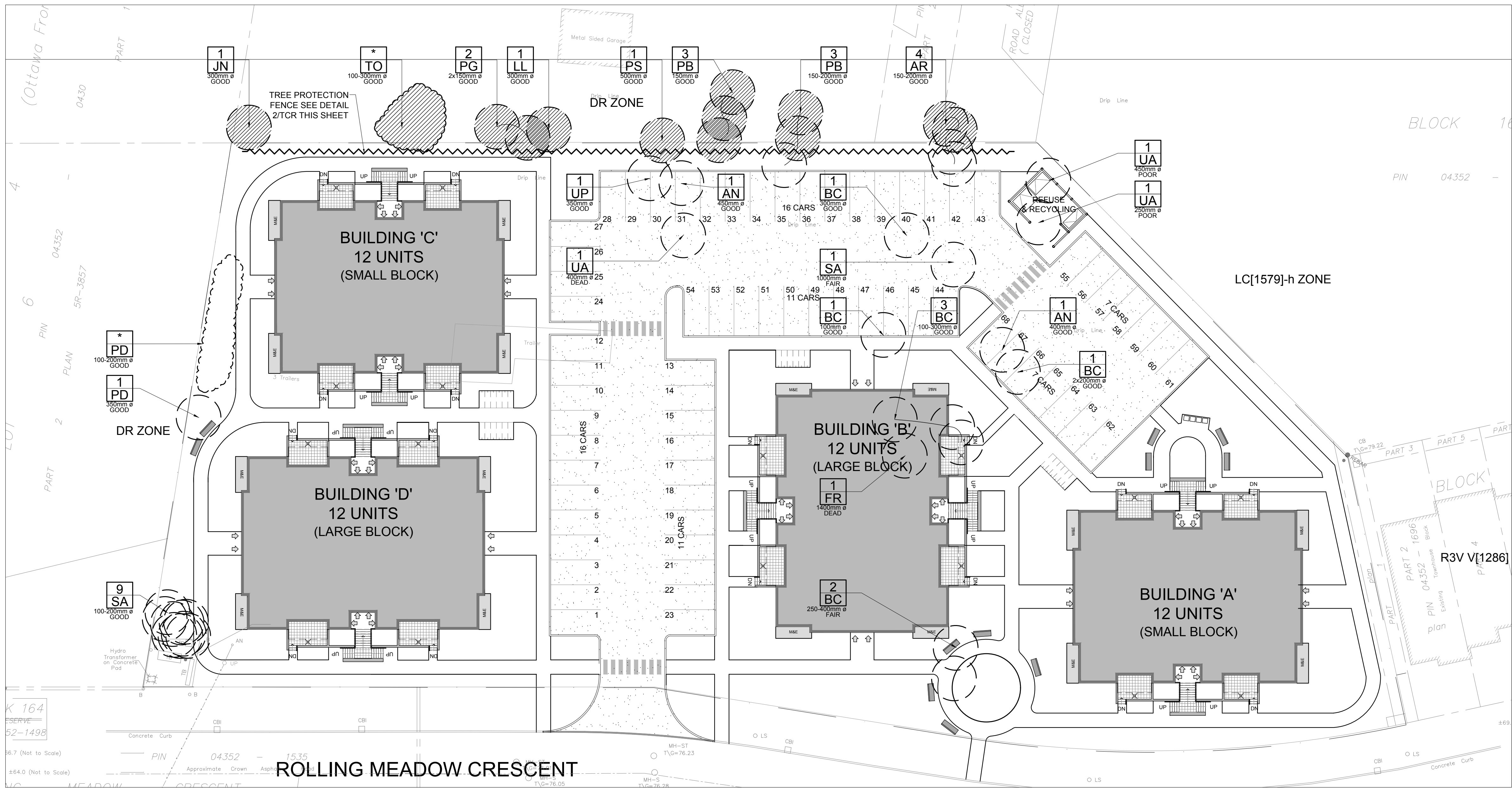
1 TREE CONSERVATION REPORT SCALE 1:250
