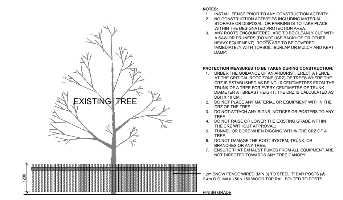
2 TREE PROTECTION FENCE SCALE: NTS
