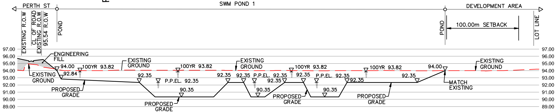
SWM POND 1 SECTION Y-Y SCALE HOR. 1:3000 VER. 1:300
