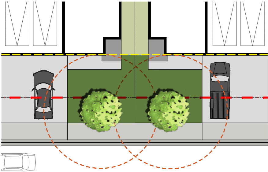
Figure 27 Tree Planting Setback - 42' Front Drive Singles
