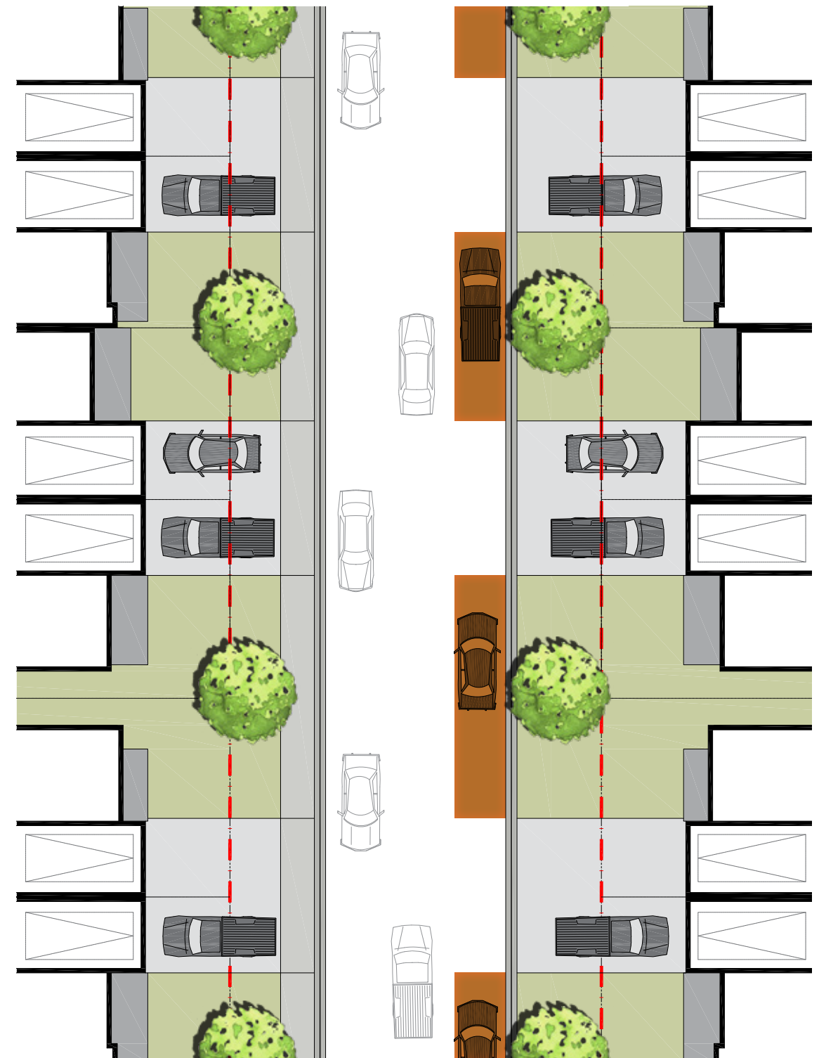
Figure 37 Front-Drive Townhomes Parking Demonstration on Local Road
