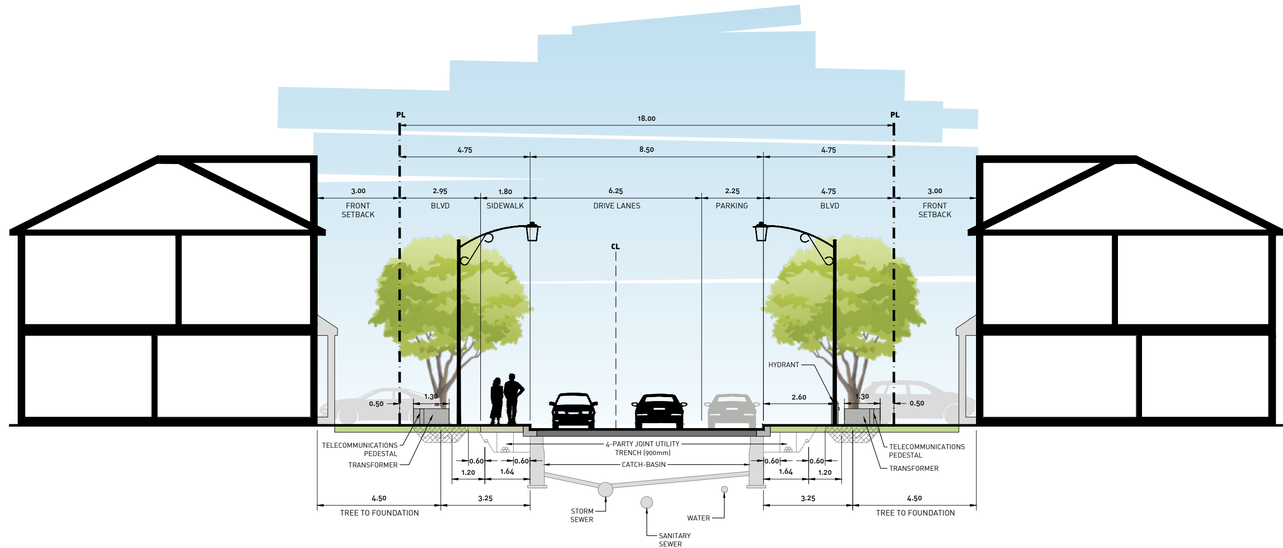
Figure 32 18.0m Local Road Right-Of-Way Section
