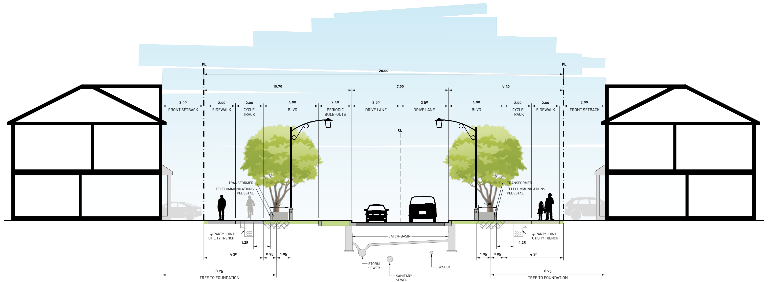
Figure 30 26.0m Collector Road (with Periodic Bulb-Out) Right-Of-Way Section
