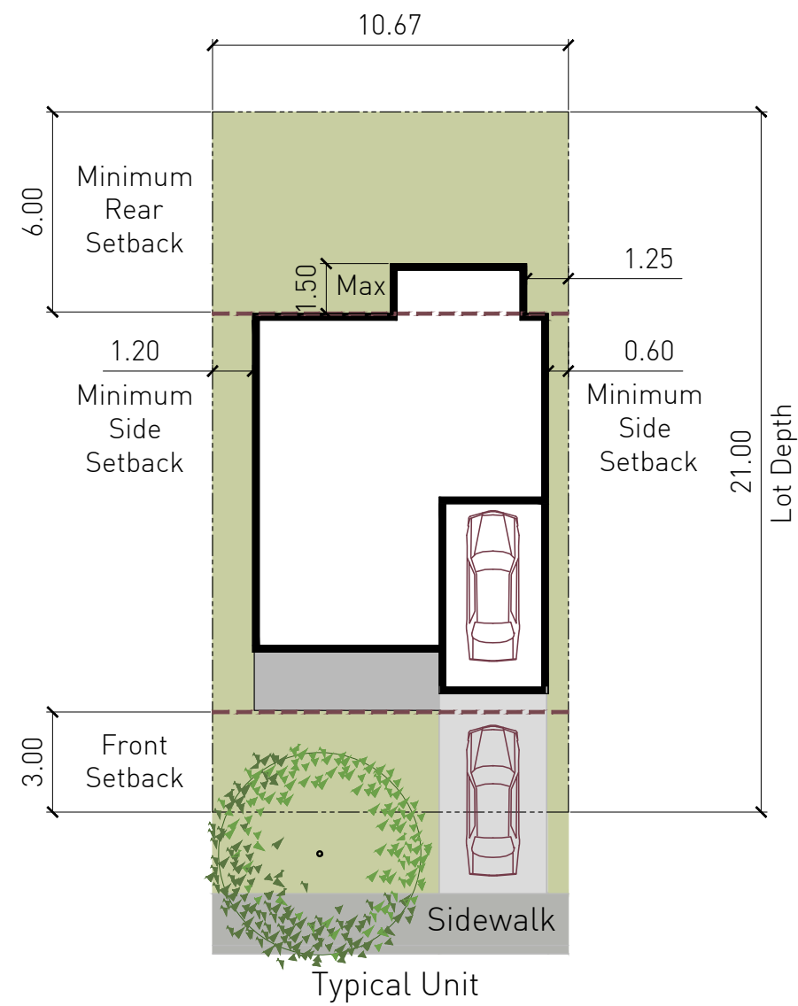
Figure 19 35' Single Detached Lotting Standard and Measurements
