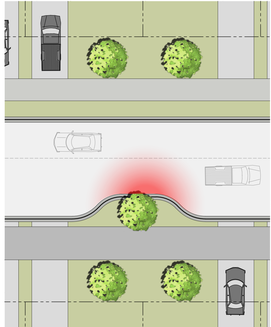
Figure 42 Mid-Block Narrowing on Collector Road
