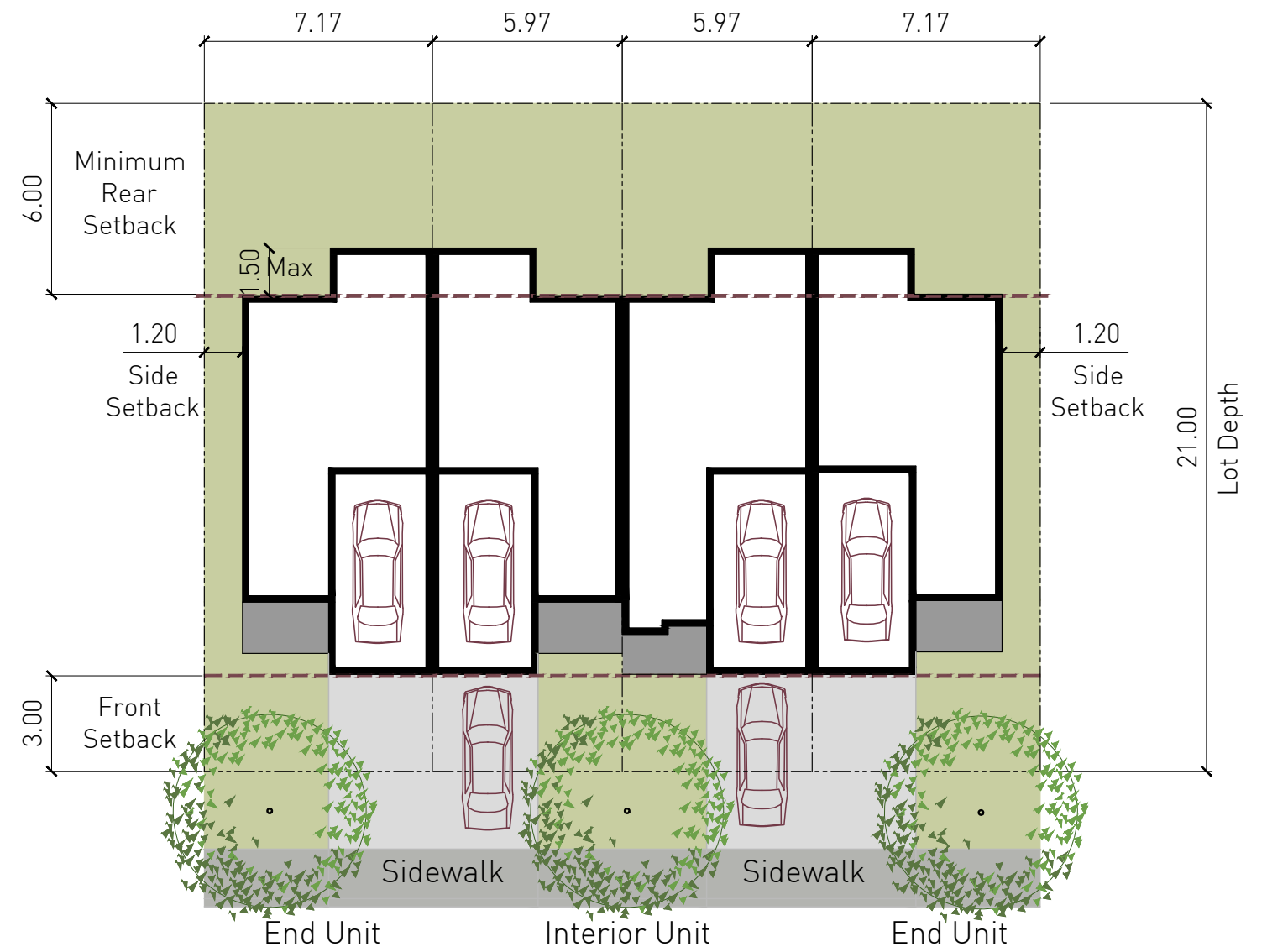
Figure 18 20' Standard Townhome Lotting Standard and Measurements
