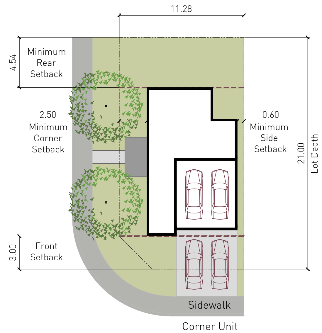
Figure 22 37' Single Detached Corner Lotting Standard and Measurements
