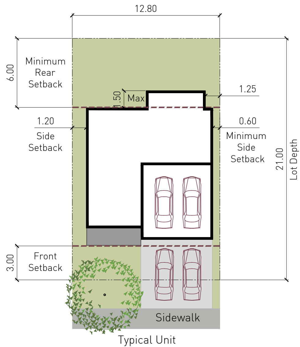
Figure 23 42' Single Detached Lotting Standard and Measurements
