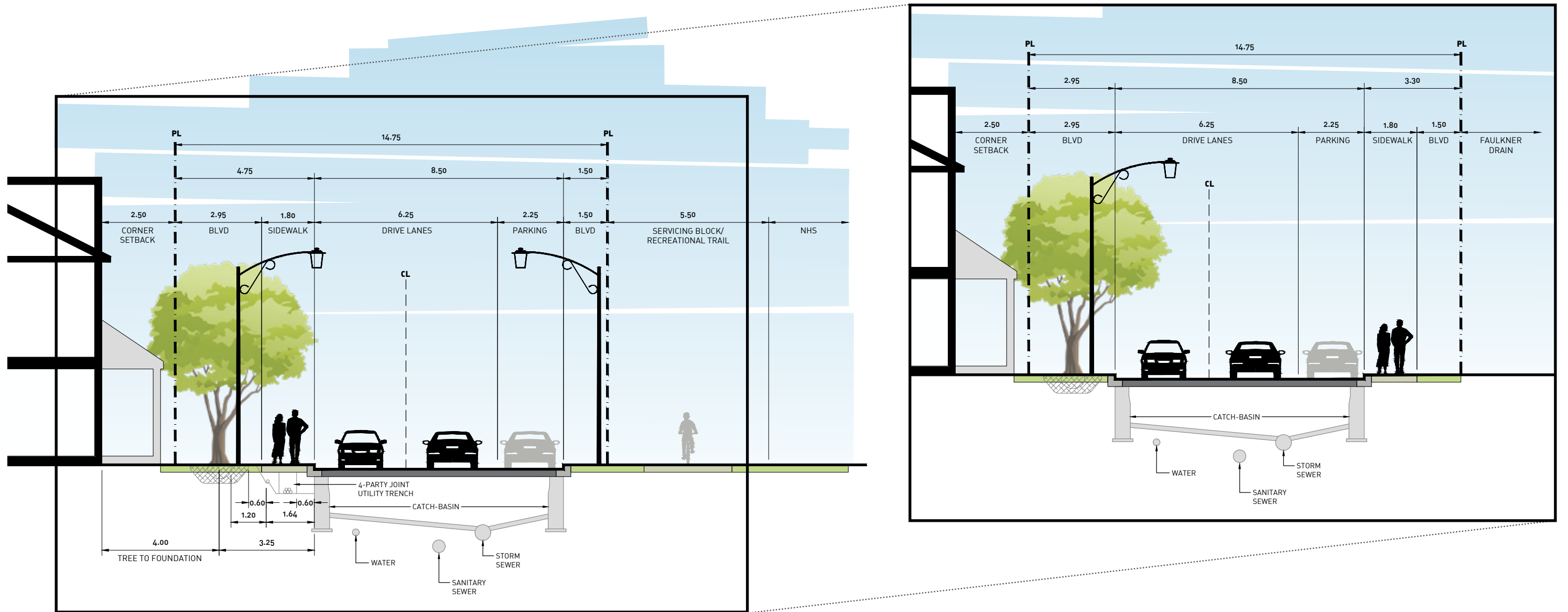
Figure 33 14.75m Window Street Right-Of-Way Section
