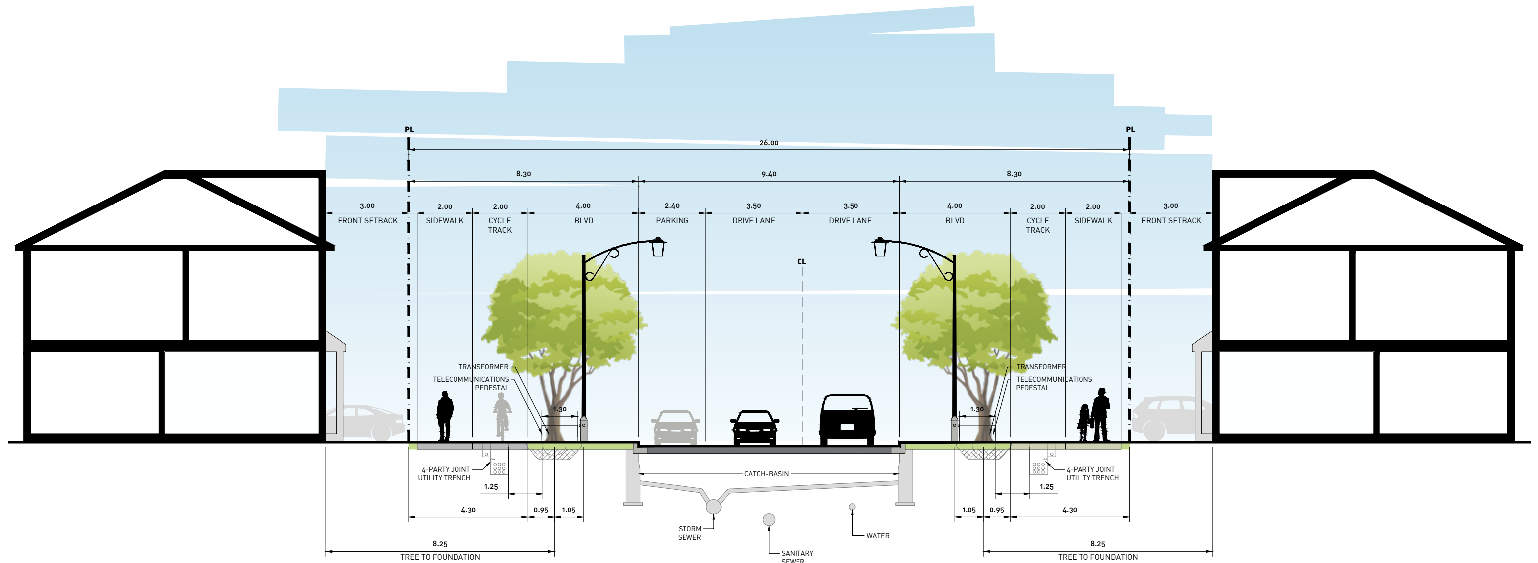
Figure 31 26.0m Collector Road (with On-Street Parking) Right-Of-Way Section
