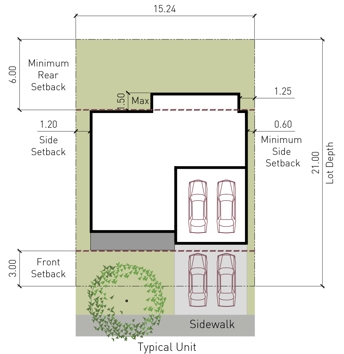
Figure 26 50' Single Detached Lotting Standard and Measurements
