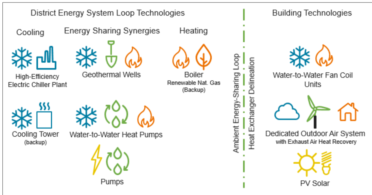
Figure 4-10: 4-Pipe District Energy System
