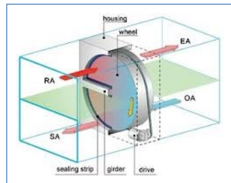
Figure: Air-to-Air Heat Recovery
