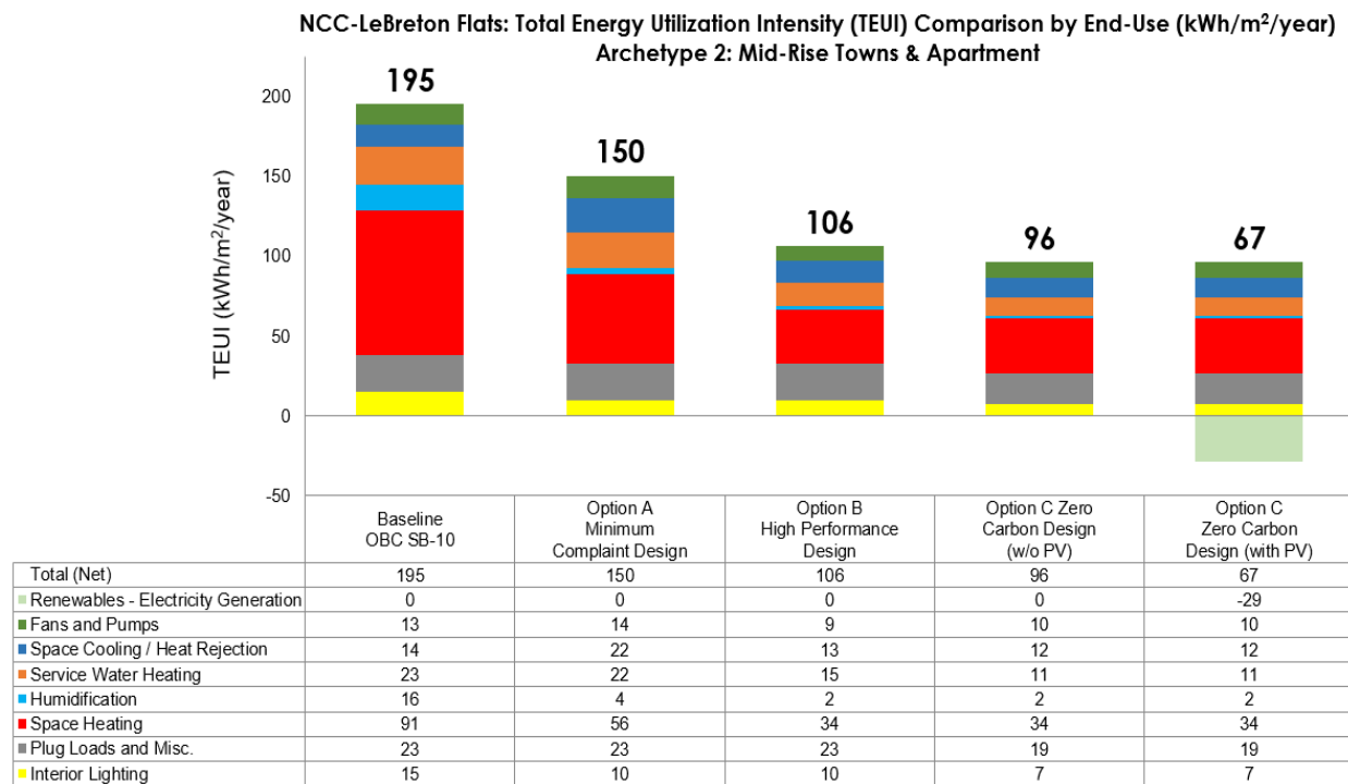
Figure 4-6: Archetype 2 End Use EUI Breakdown
