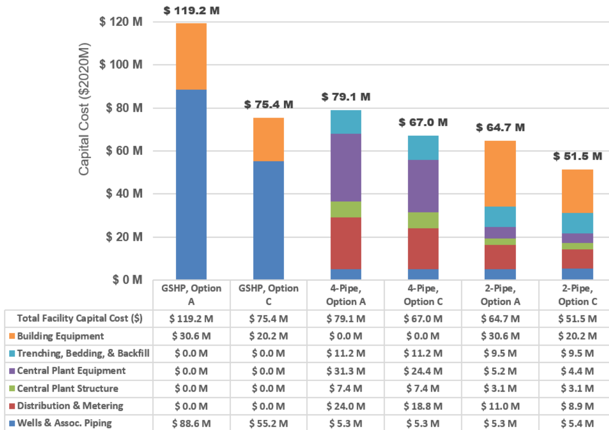
Figure 5-1: HVAC Capital Cost Breakdown ($2020M)
