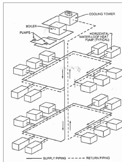
Figure: Distributed Heat Pumps
