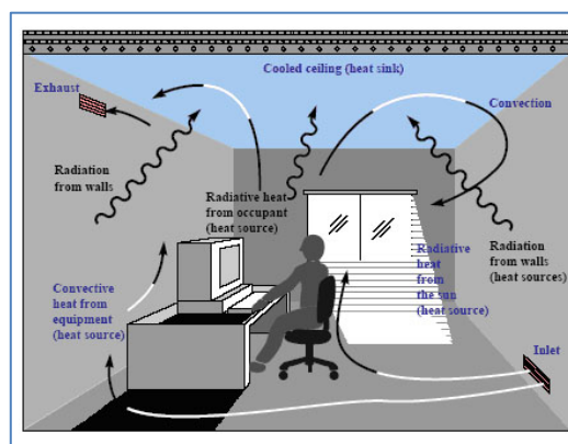
Figure: Displacement Ventilation
