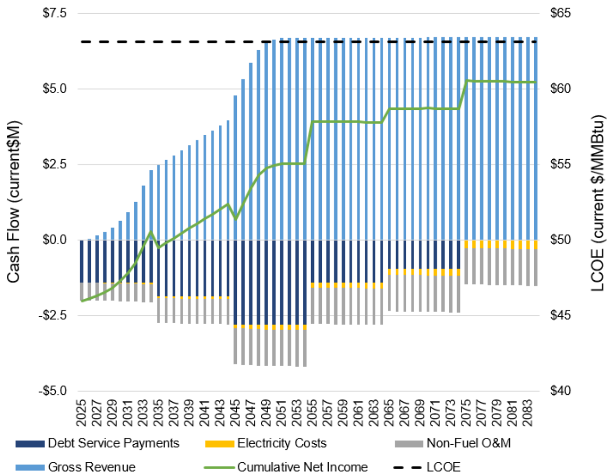
Figure 5-5: Cash Flow 2-Pipe Option C (Current $M)
