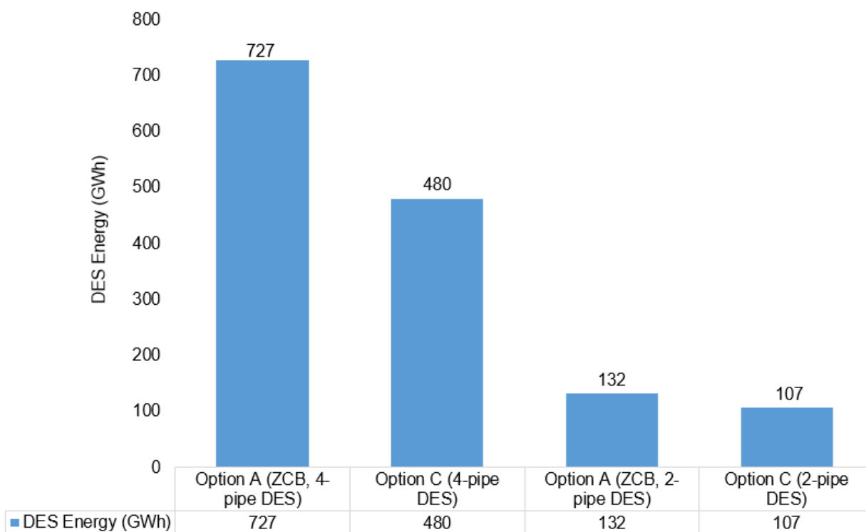
Figure 4-12: DES Space Heating and Space Cooling Energy
