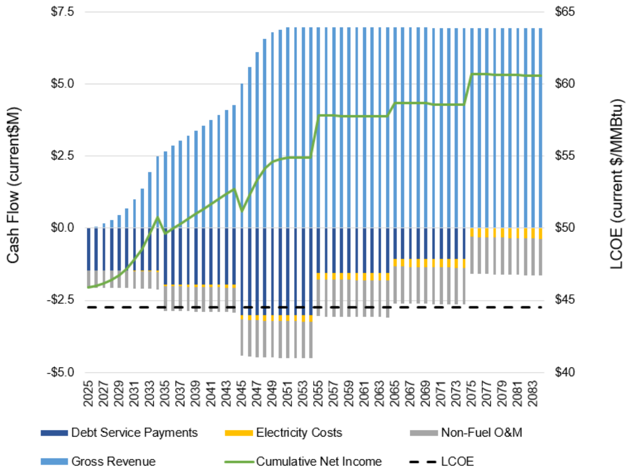
Figure 5-4: Cash Flow 2-Pipe Option A (Current $M)
