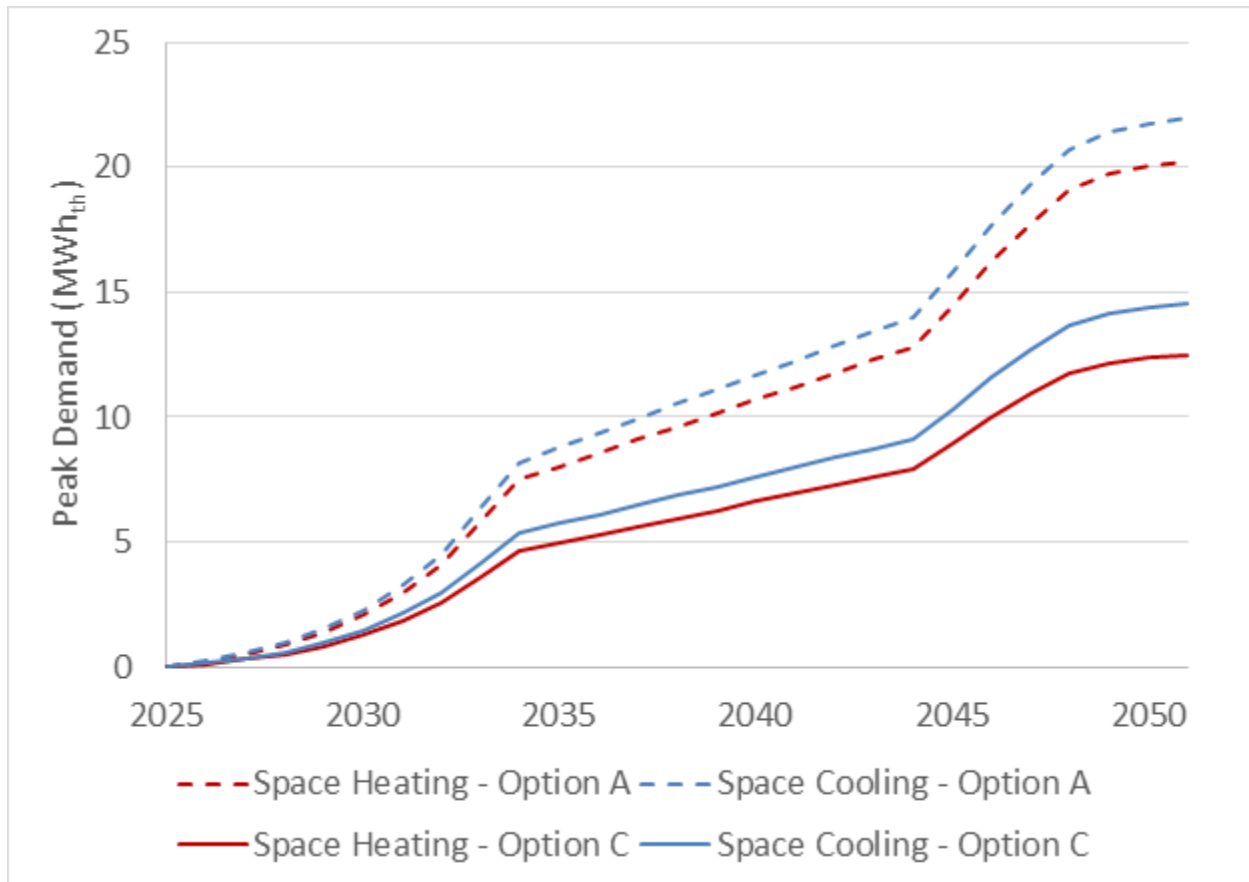
Figure 4-9: LeBreton Flats Thermal Loads
