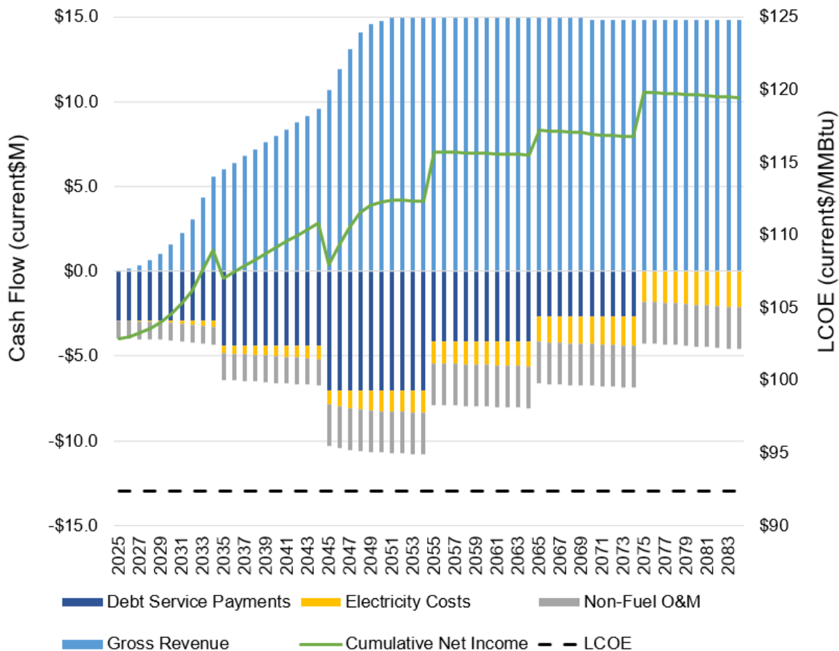
Figure 5-2: Cash Flow 4-Pipe Option A (Current $M)
