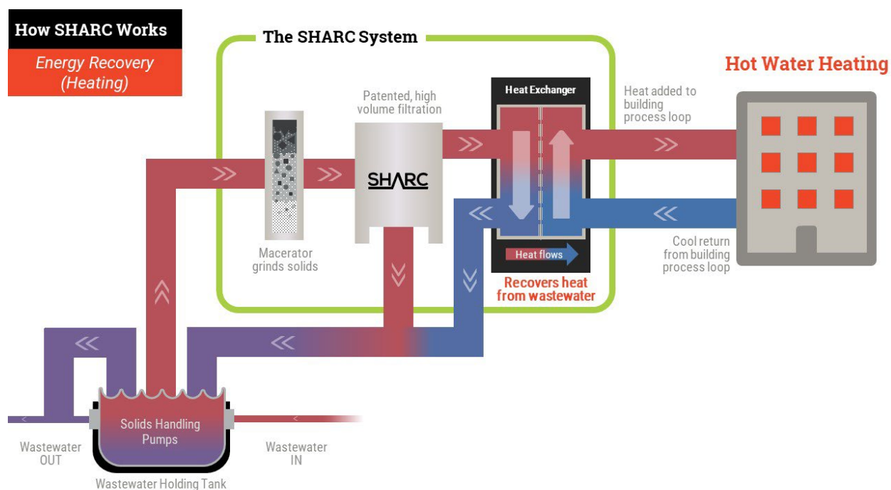
Figure 3-9: SHARC Sewer Heat Recovery System 11
