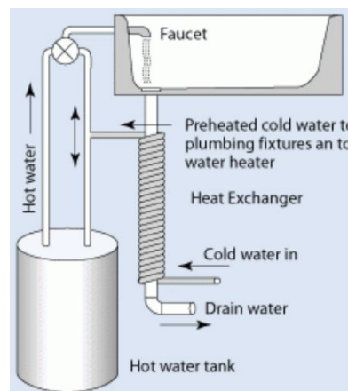
Figure 4-2: Drain Water Heat Recovery System
