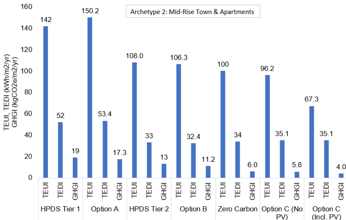
Figure 4-4: Archetype 2 Performance Metrics Achieved vs. Benchmarks
