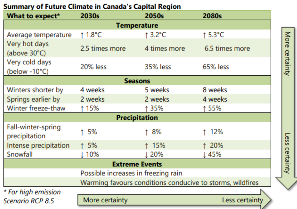
Figure 3-5 Summary of Future Climate in Canada's Capital Region 7
