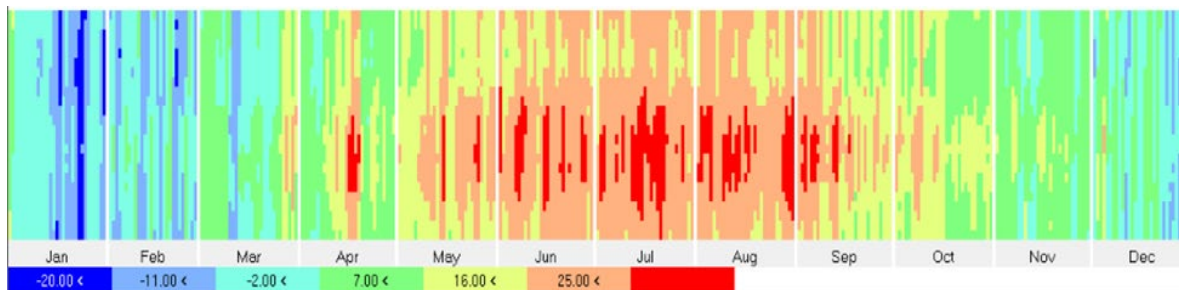
Figure 3-3: CWEC 2016 – Present Climate (Ottawa) 5
