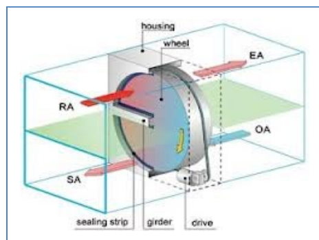
Figure 4-1: Air-to-Air Energy Recovery
