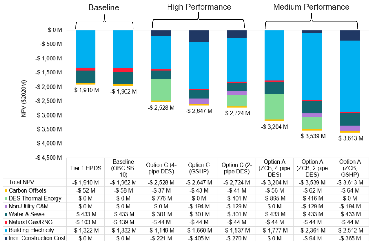
Figure 5-6: Net Present Value of Urban Scenarios
