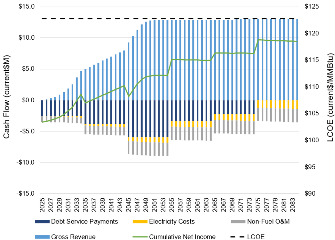
Figure 5-3: Cash Flow 4-Pipe Option C (Current $M)
