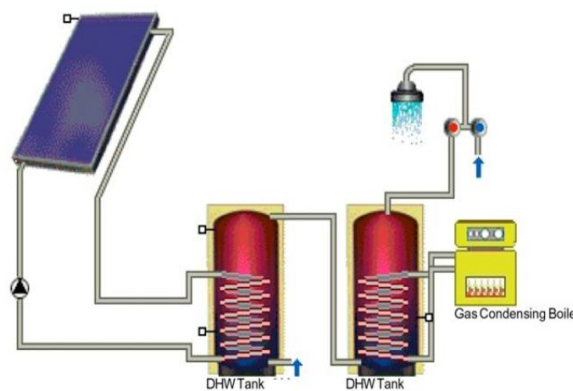
Figure: Solar Thermal System
