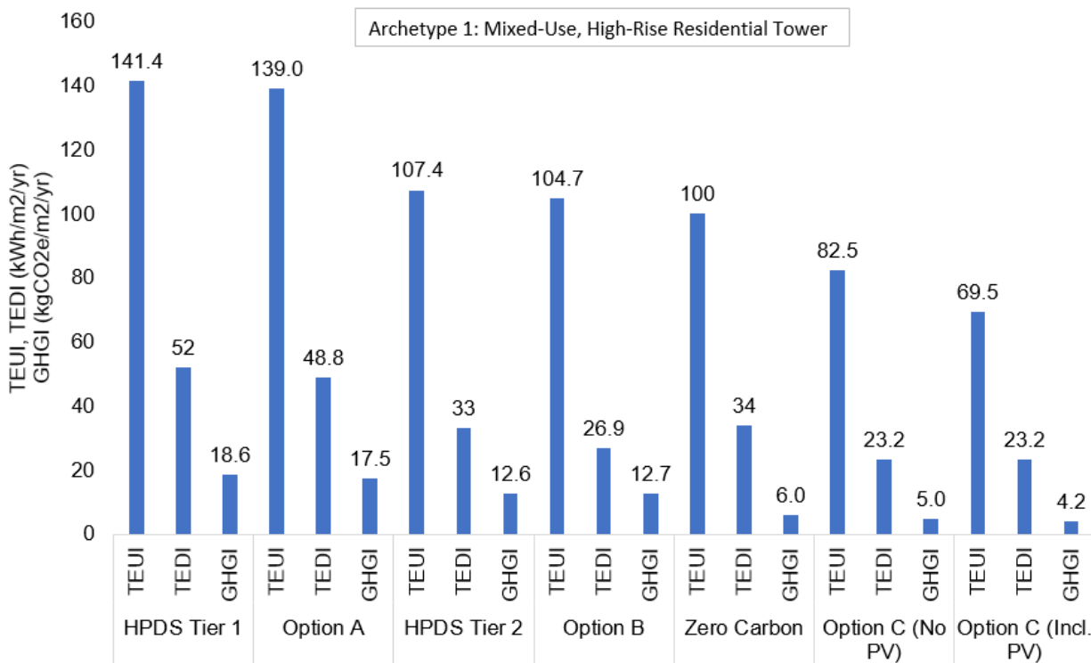
Figure 4-3: Archetype 1 Performance Metrics Achieved vs. Benchmarks
