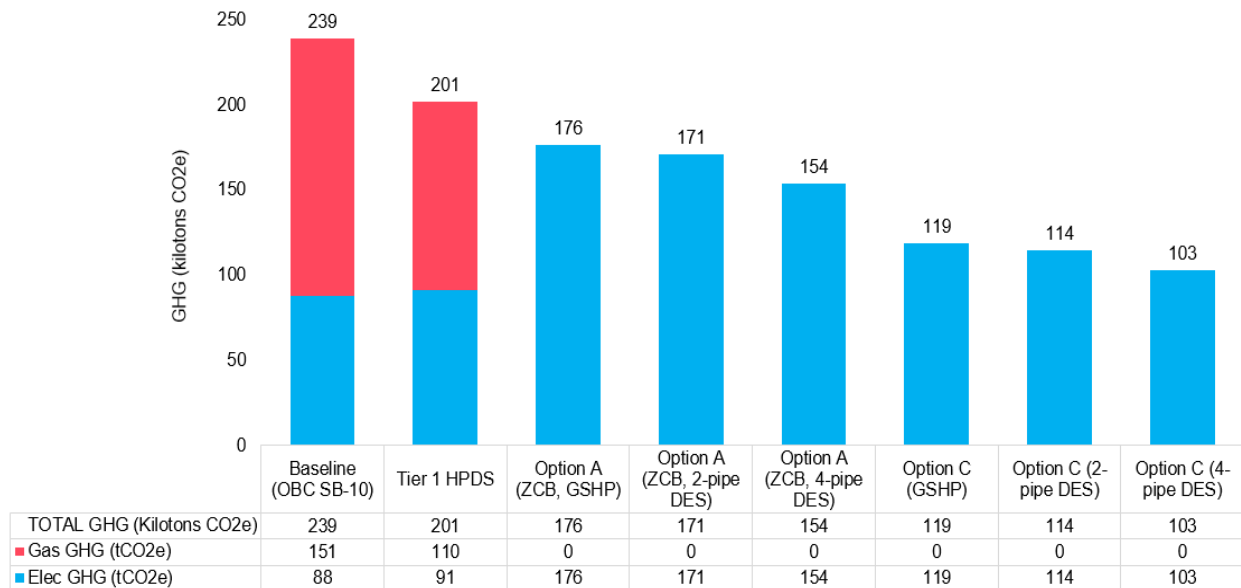
Figure 4-15: Total GHG Emissions
