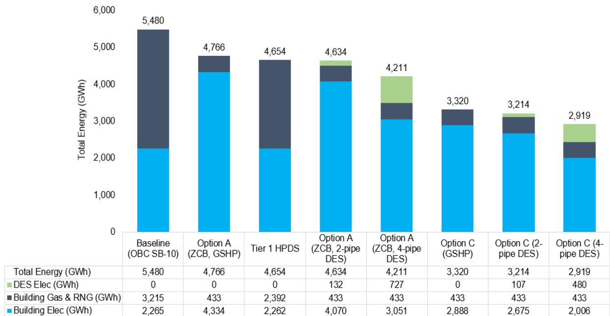
Figure 4-14: Total Urban Energy Use
