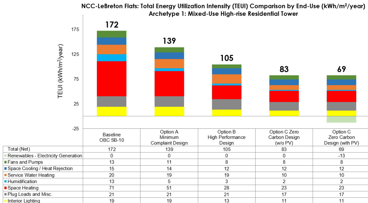
Figure 4-5: Archetype 1 End Use EUI Breakdown
