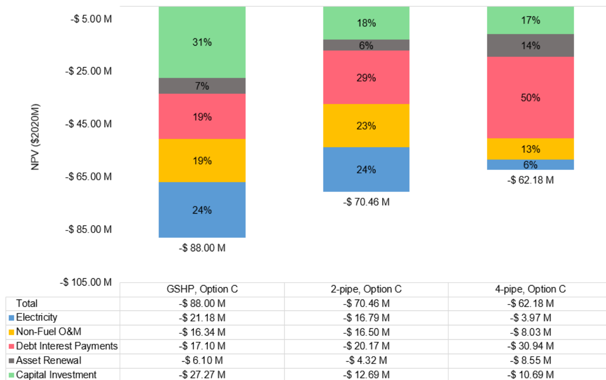
Figure 5-7: Net Present Value of HVAC Options
