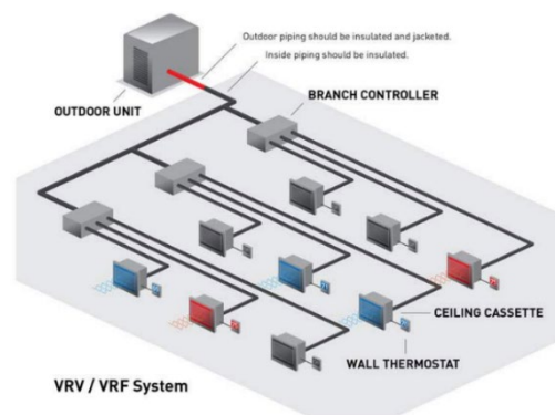
Figure: VRF-HR System
