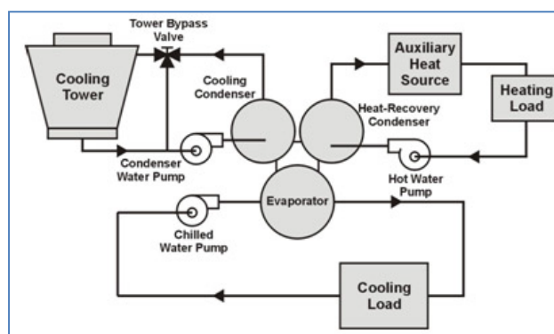
Figure: Heat Recovery Chiller
