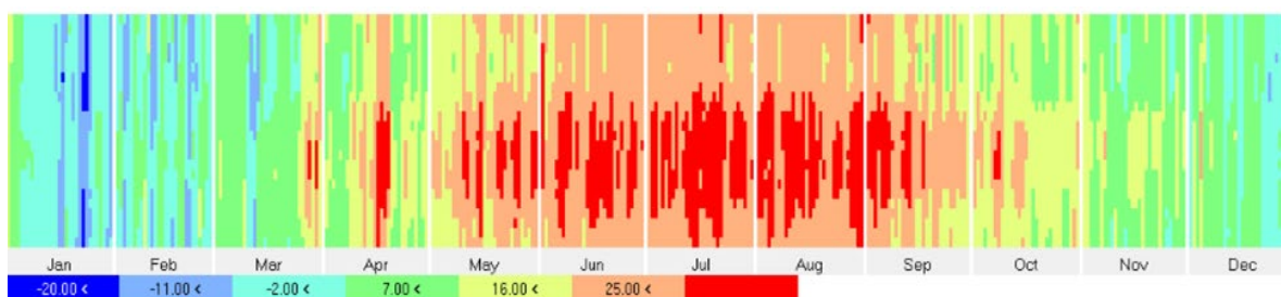
Figure 3-4: RCP 8.5 – 2031 to 2050 – 90th Percentile (Ottawa) 6
