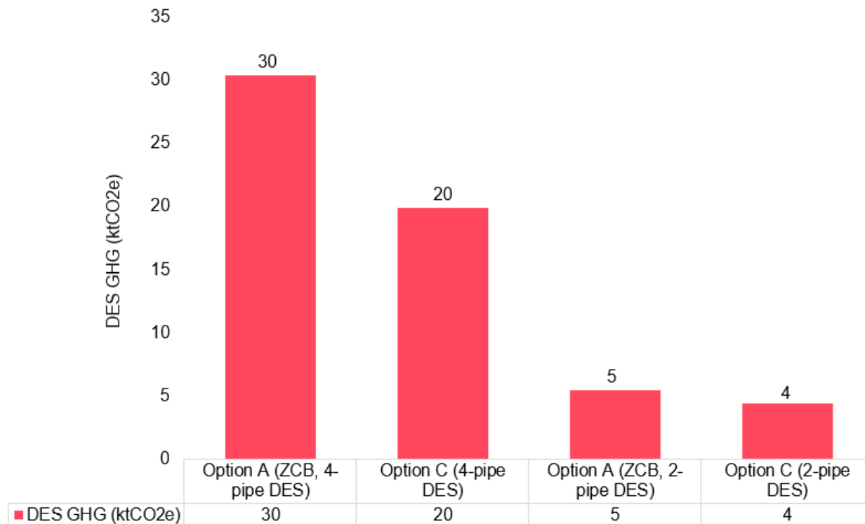
Figure 4-13: DES Space Heating and Space Cooling GHG Emissions
