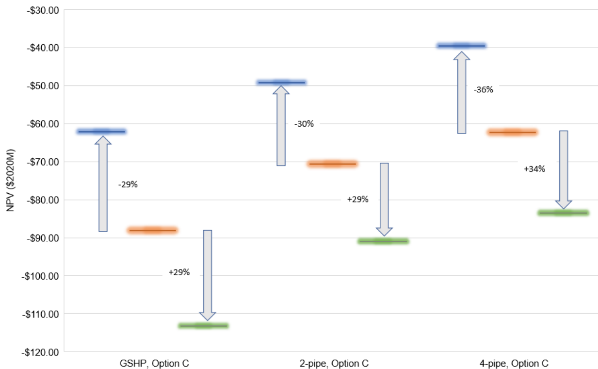
Figure 5-8: Effect of Sensitivity Analysis on HVAC Options
