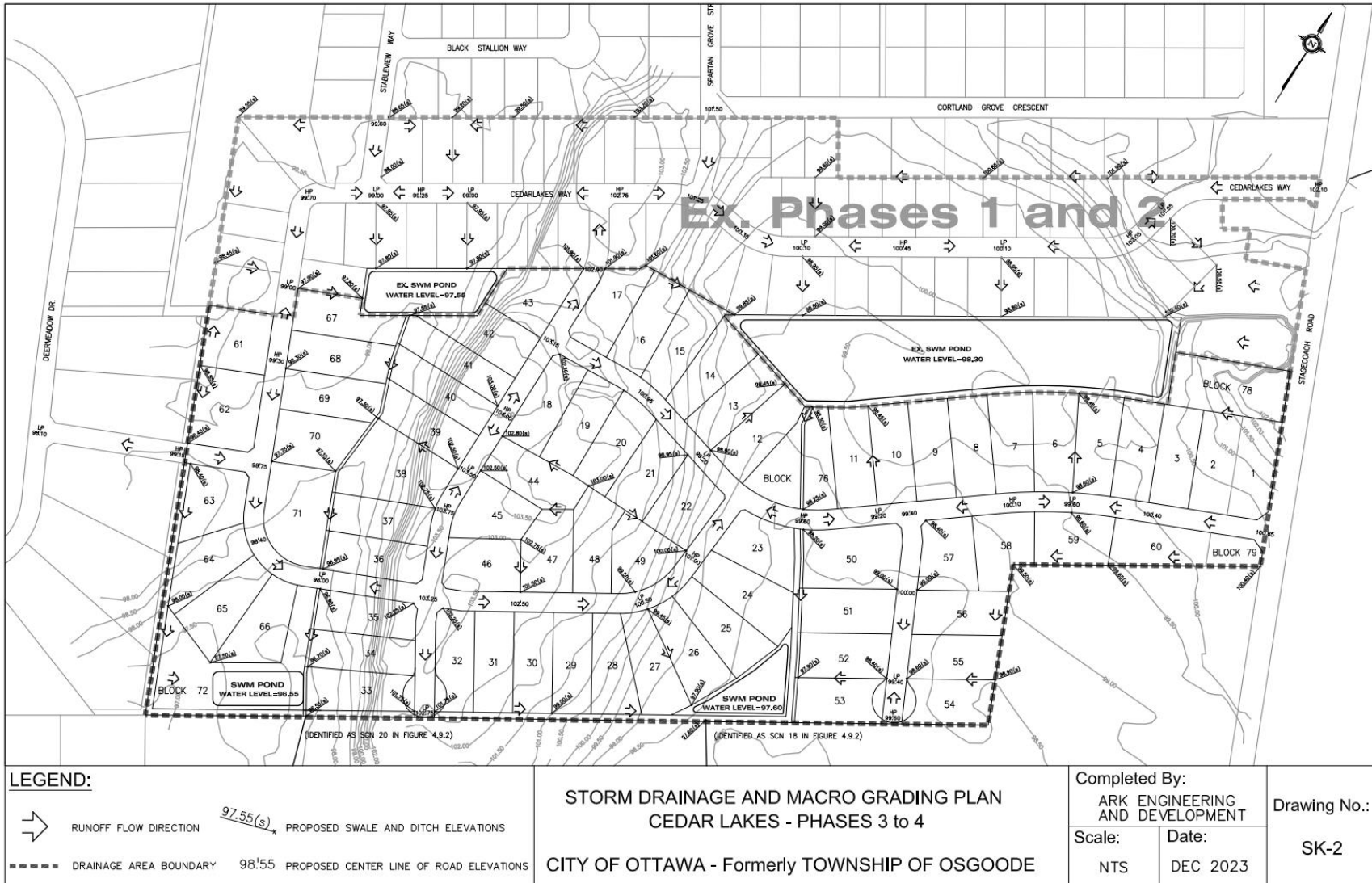
FIGURE 2: SITE PLAN
