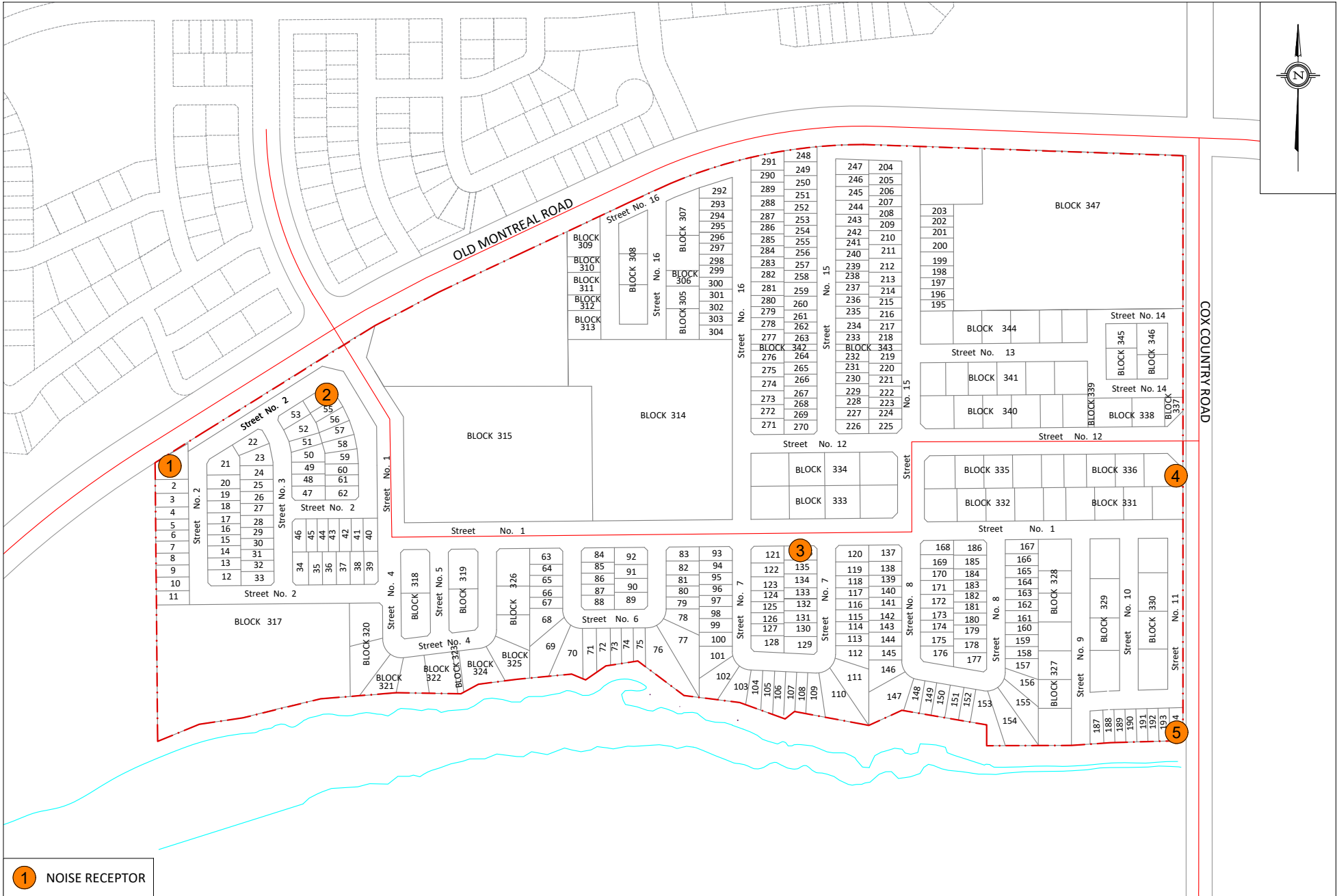
FIGURE 2: NOISE SOURCE AND RECEPTOR LOCATIONS
