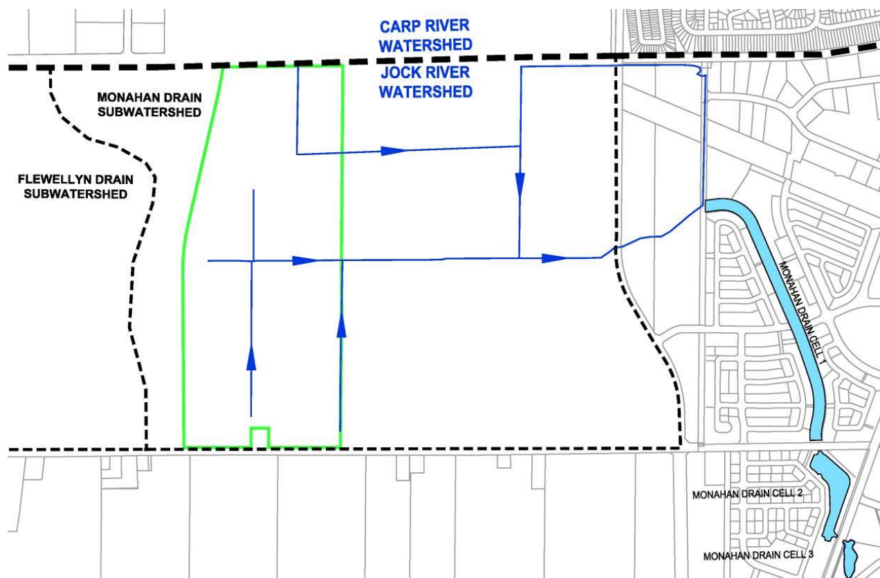
Figure 5: Existing Watershed Boundaries
