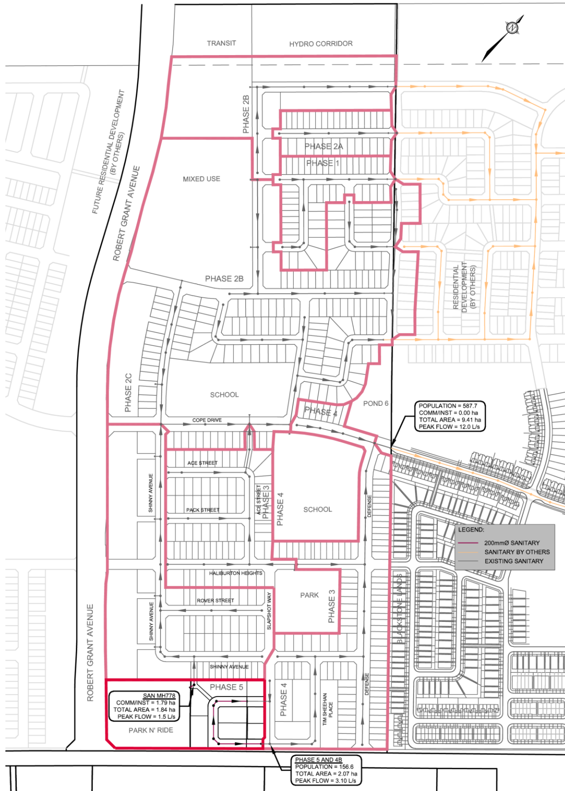
Figure 4: Sanitary Sewer Network
