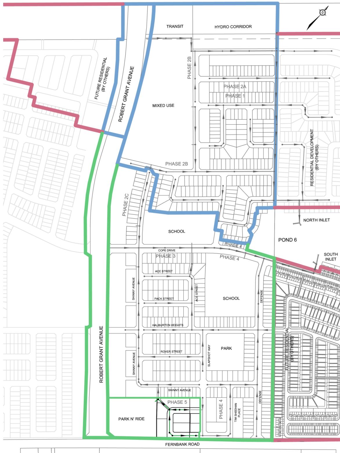
Figure 6: Storm Sewer Network
