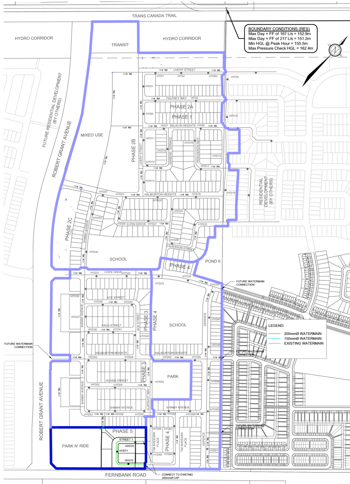
Figure 8: Watermain Layout
