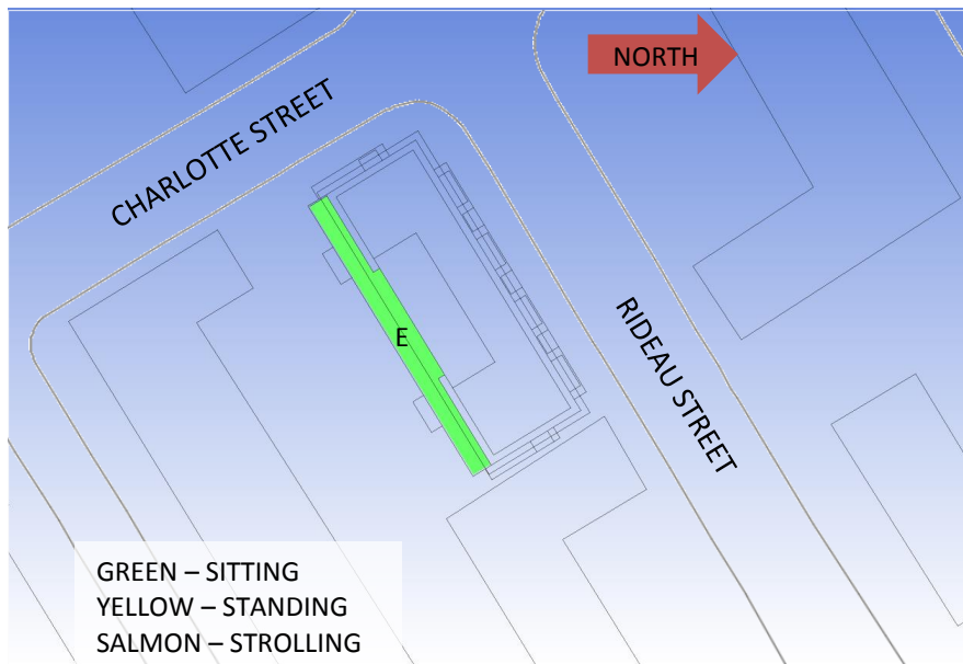
FIGURE 5B: AUTUMN – LEVEL SEVEN AMENITY TERRACE PEDESTRIAN WIND CONDITIONS
