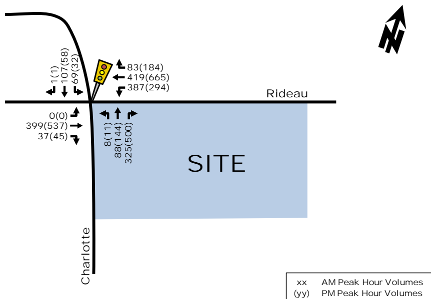
Figure 4: Existing Peak Hour Traffic Volumes
