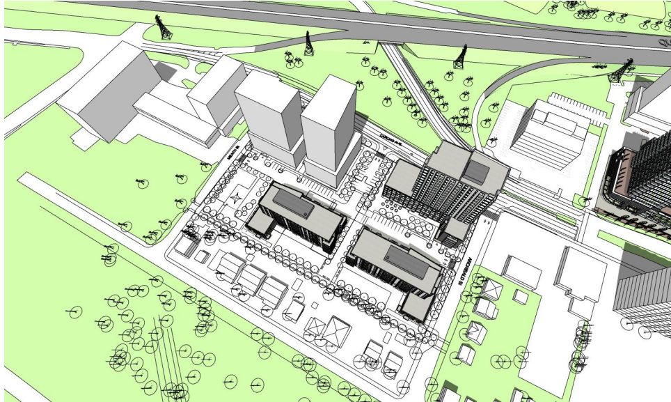
Noon Short shadow projections of Buildings D & E over immediate outdoor area No shadow casted on south facades of all buildings
