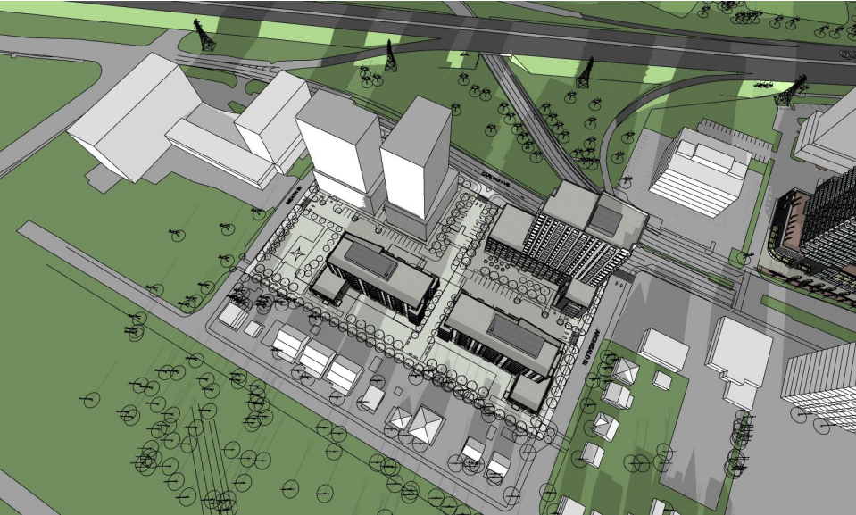
10:00 am Long shadow projections of Buildings D & E over outdoor parking area Long shadow projections of neighboring buildings over backside of Buildings D
