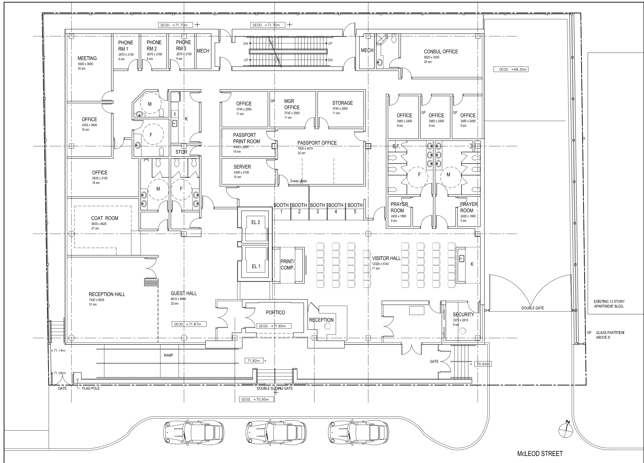
GROUND FLOOR PLAN FEB 2013
