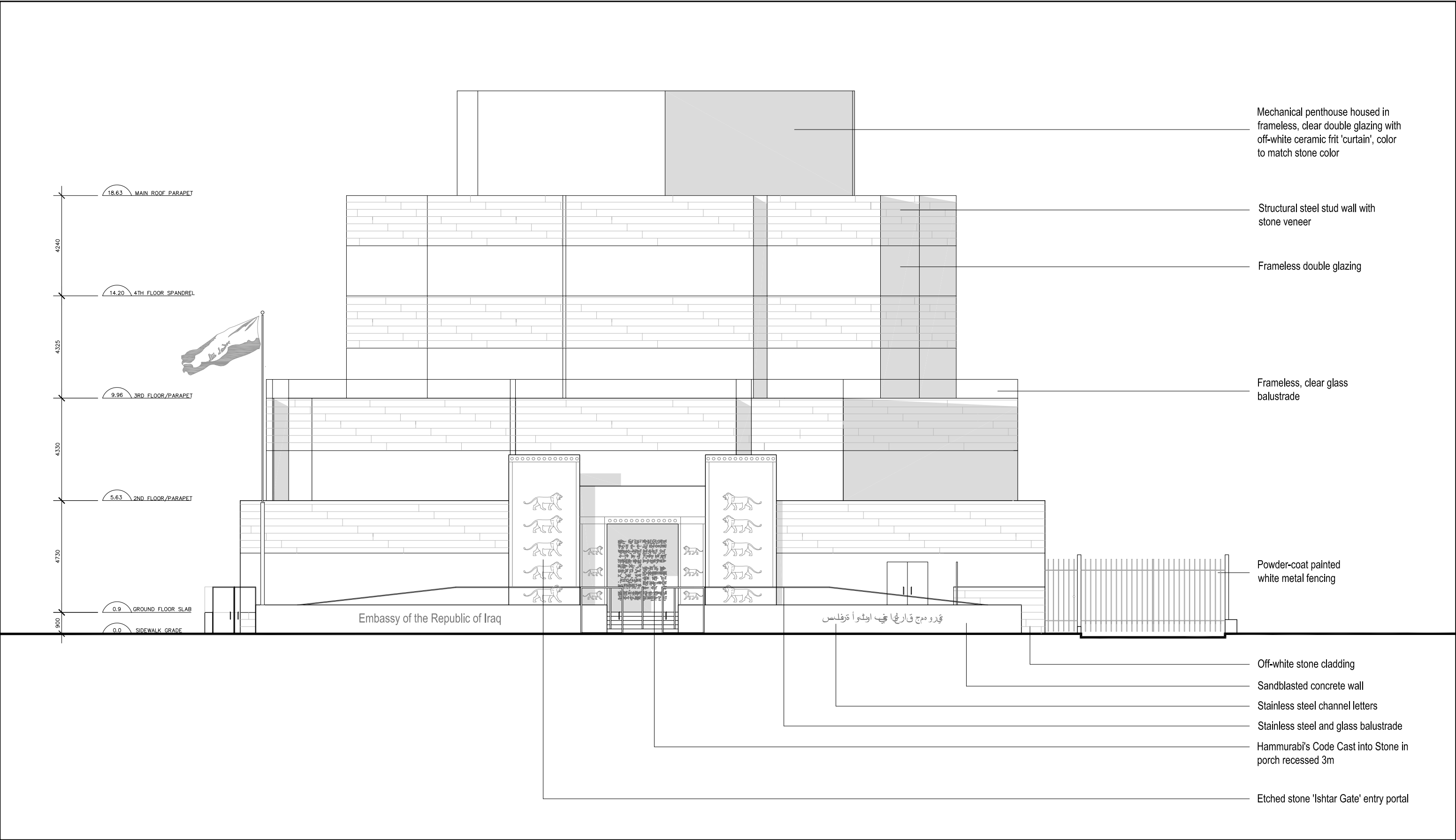
SOUTH/ FRONT ELEVATION
