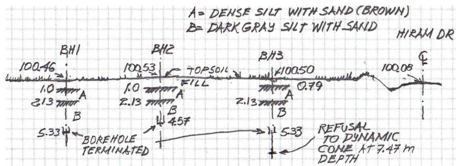
Figure 2: Schematic cross section
