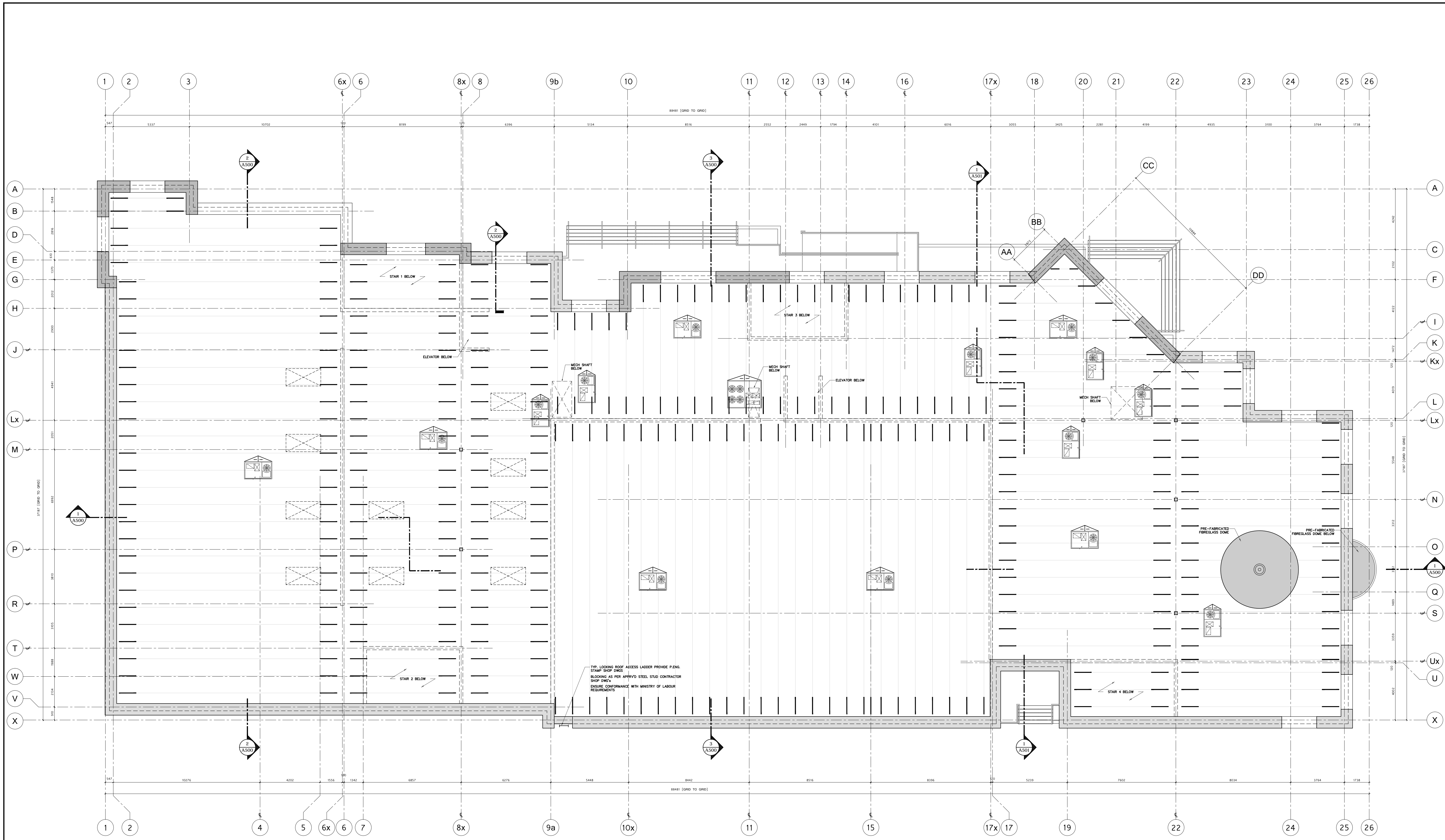
1 ROOF PLAN A203 SCALE 1:125
