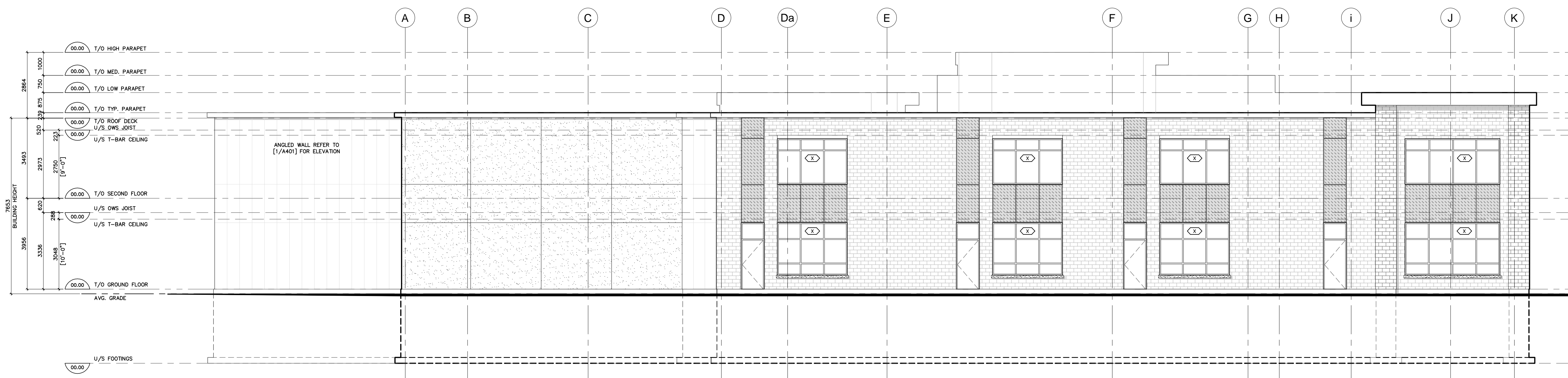
2 SOUTH [SIDE] ELEVATION SCALE 1:100
