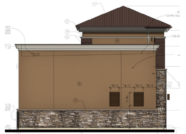
South Elevation
