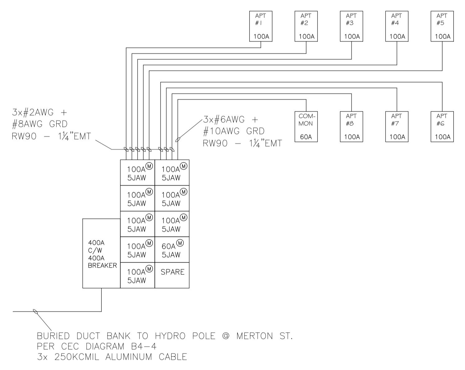
1 SITE FEED SINGLE LINE DIAGRAM SPE1 N.T.S.
