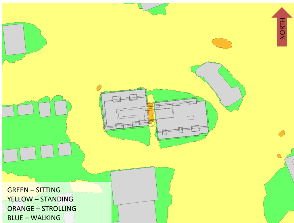
FIGURE 3: SPRING – GRADE-LEVEL PEDESTRIAN WIND CONDITIONS
