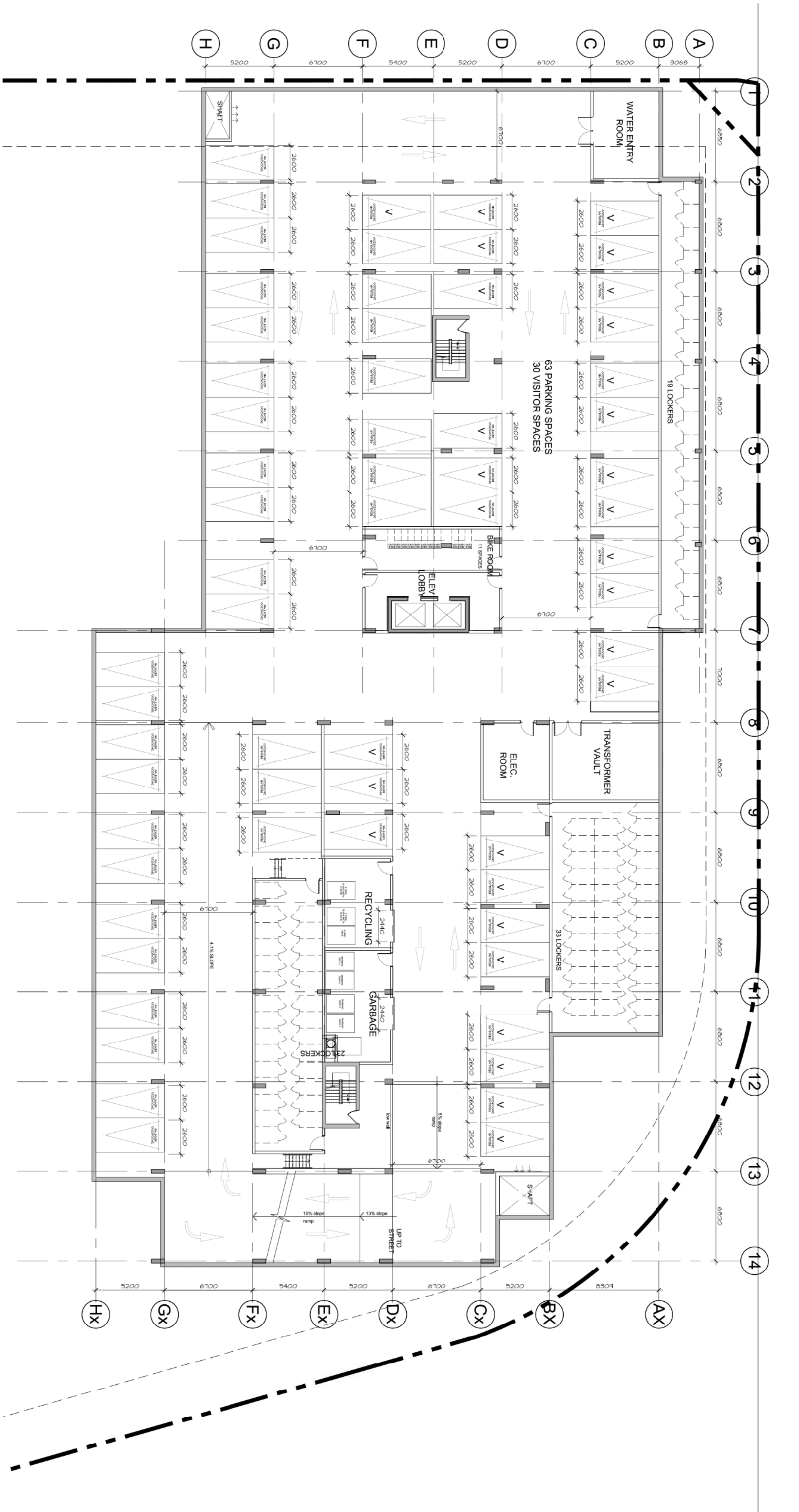
1 FLOOR PLAN - LEVEL P1 A1.02 1:150
