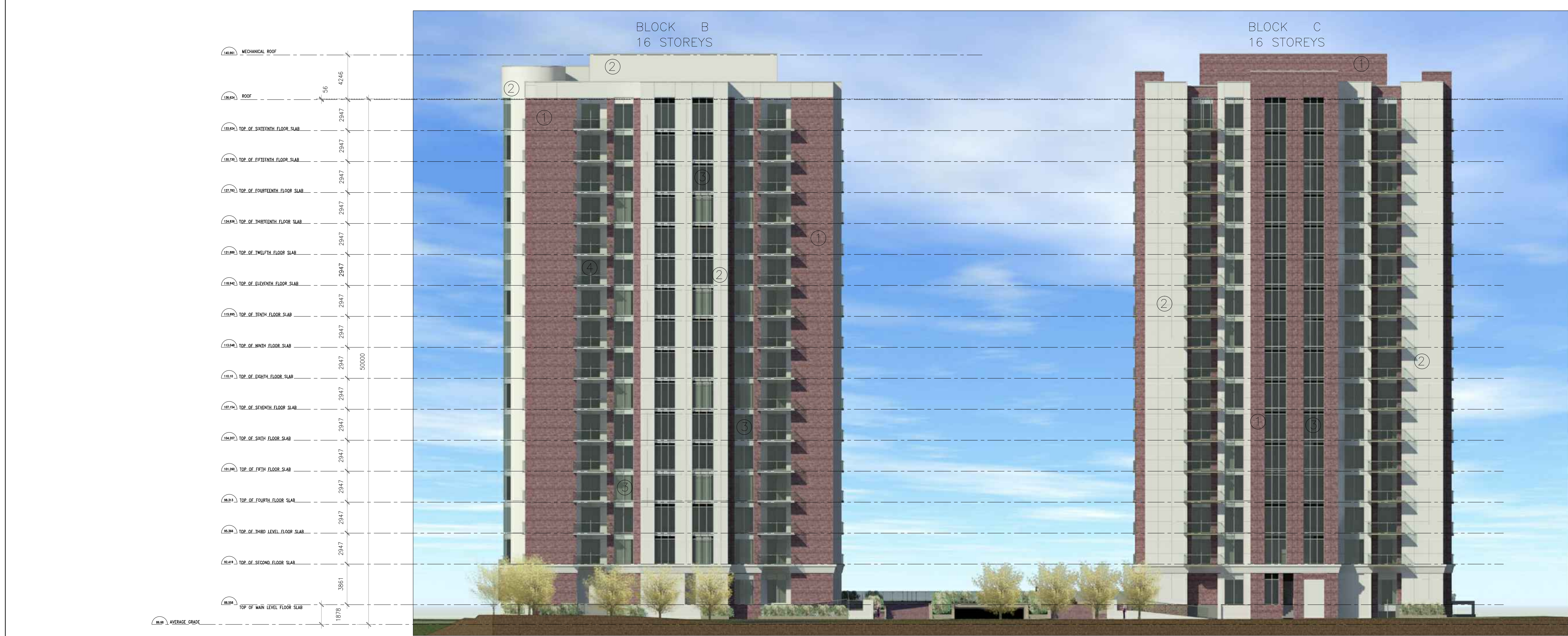
1 ELEVATION EAST AE.02 1:175
