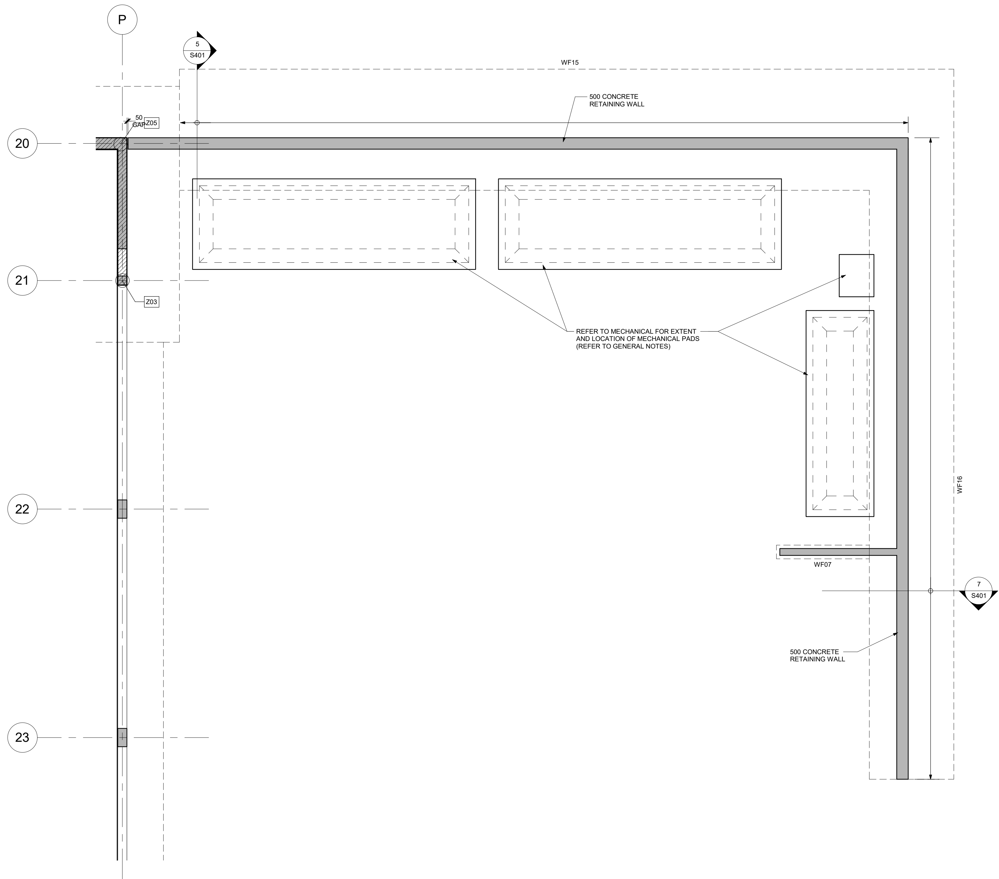
COURTYARD PLAN 1 : 100
