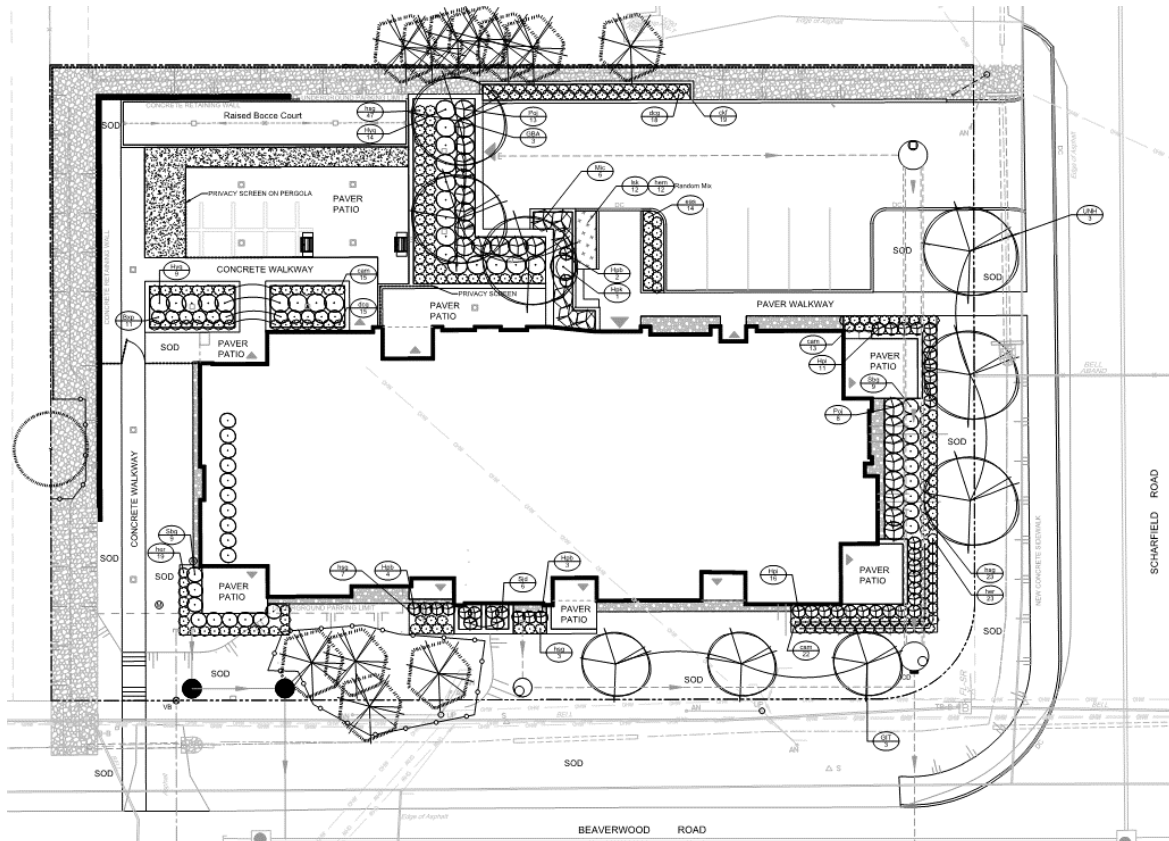
Figure 11. Landscape Plan
