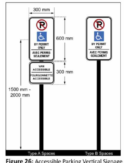
Figure 26: Accessible Parking Vertical Signage
