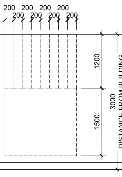
BICYCLE PARKING DIMENSIONS
