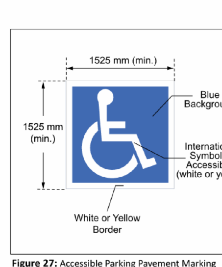
Figure 27: Accessible Parking Pavement Marking
