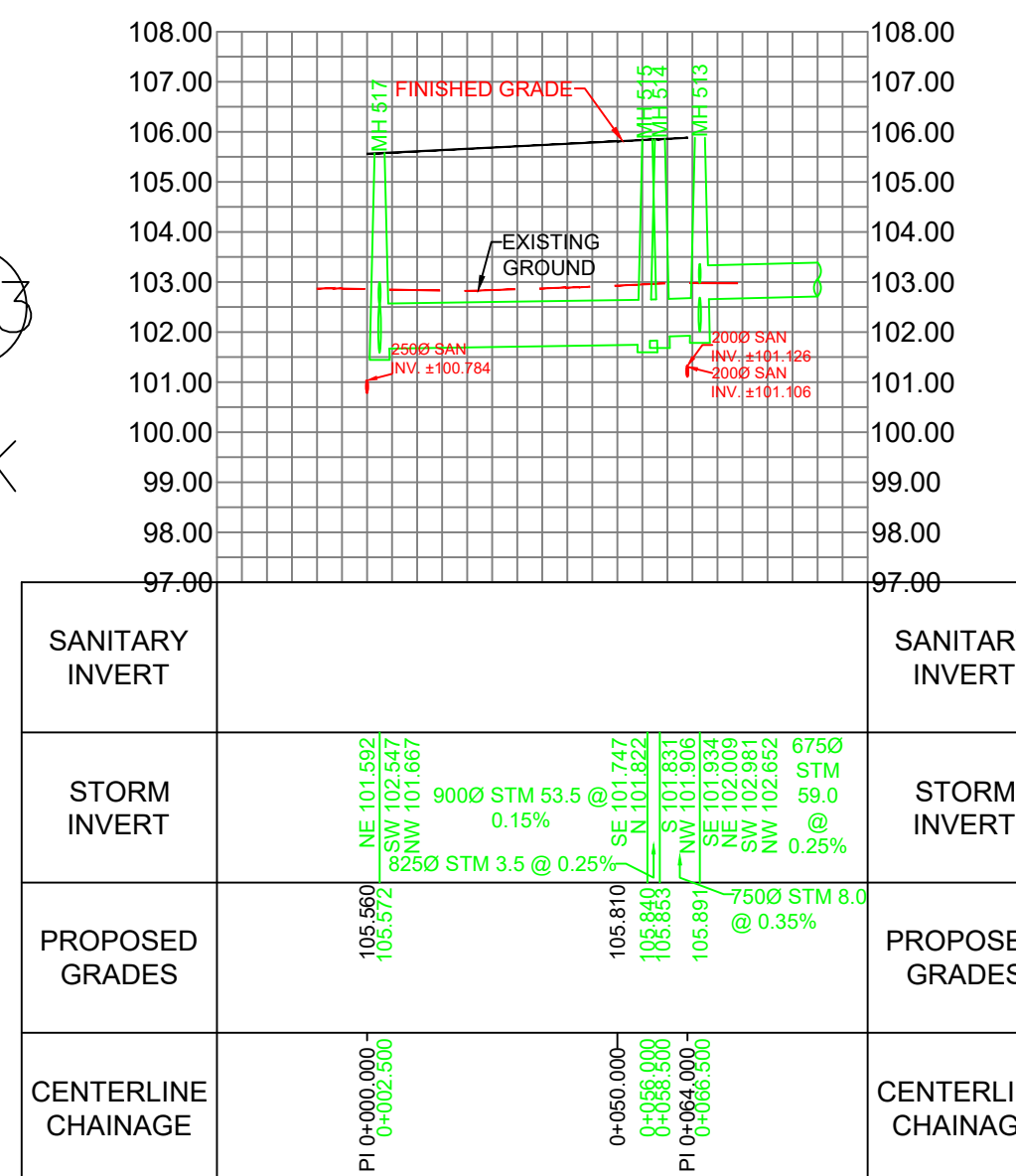
503 SERVICING BLOCK
