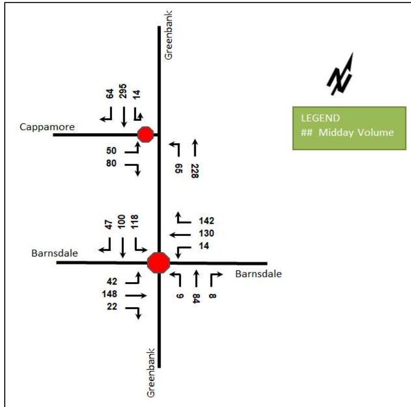
Figure 10: Existing Traffic Counts- Friday Midday
