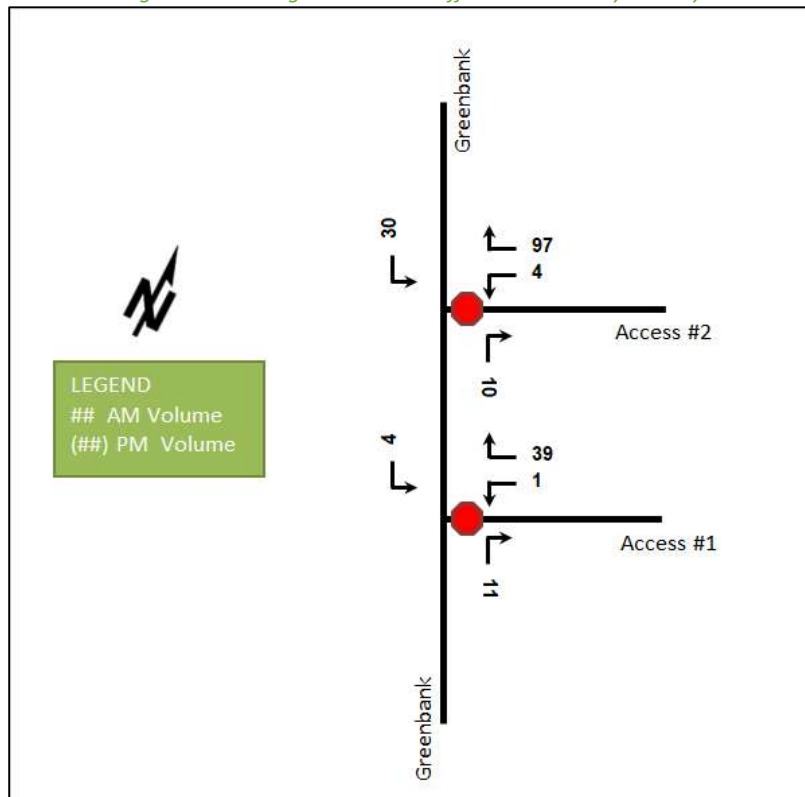
Figure 12: Existing Site Access Traffic Counts- Friday MIDDAY
