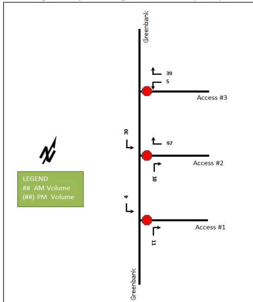
Figure 13: Proposed Site Traffic Redistribution- Friday Midday
