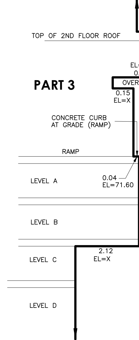
SECTION "A-A"
