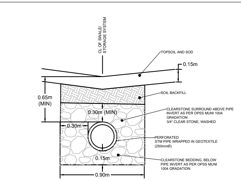
PERFERATED PIPE TRENCH DETAIL N.T.S.
