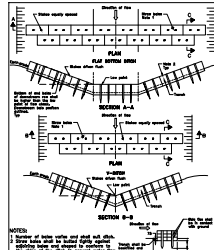
DESIGN THROUGH STANDARD DRAWING No. 202-110-1 STRAW BALE FLOW CHECK DAM
