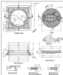
STANDARD CIRCULAR SANITARY & COMBINED MAINTENANCE HOLE COVER
