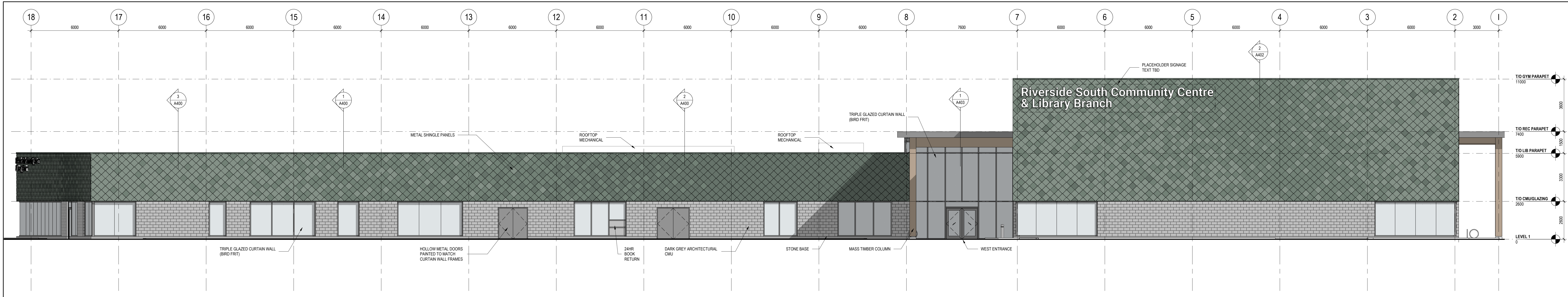
2 WEST ELEVATION A300 1:100
