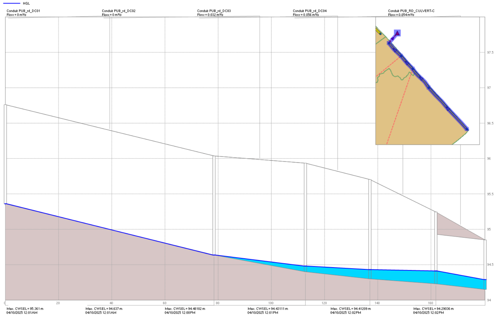
Figure 5: Profile public ditch to outfall C pre-development 2y storm event
