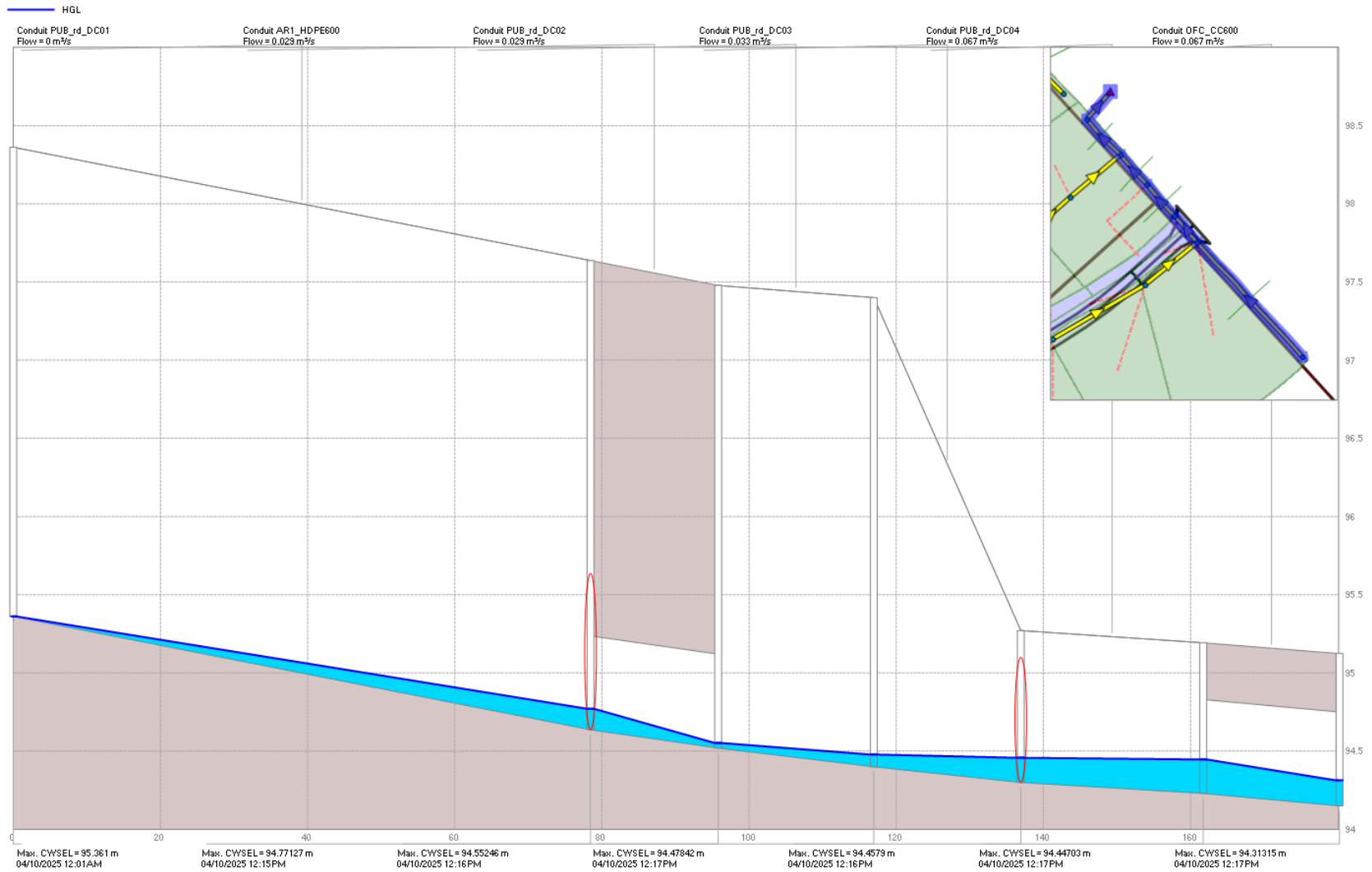
Figure 6: Profile public ditch to outfall C post-development 2y storm event
