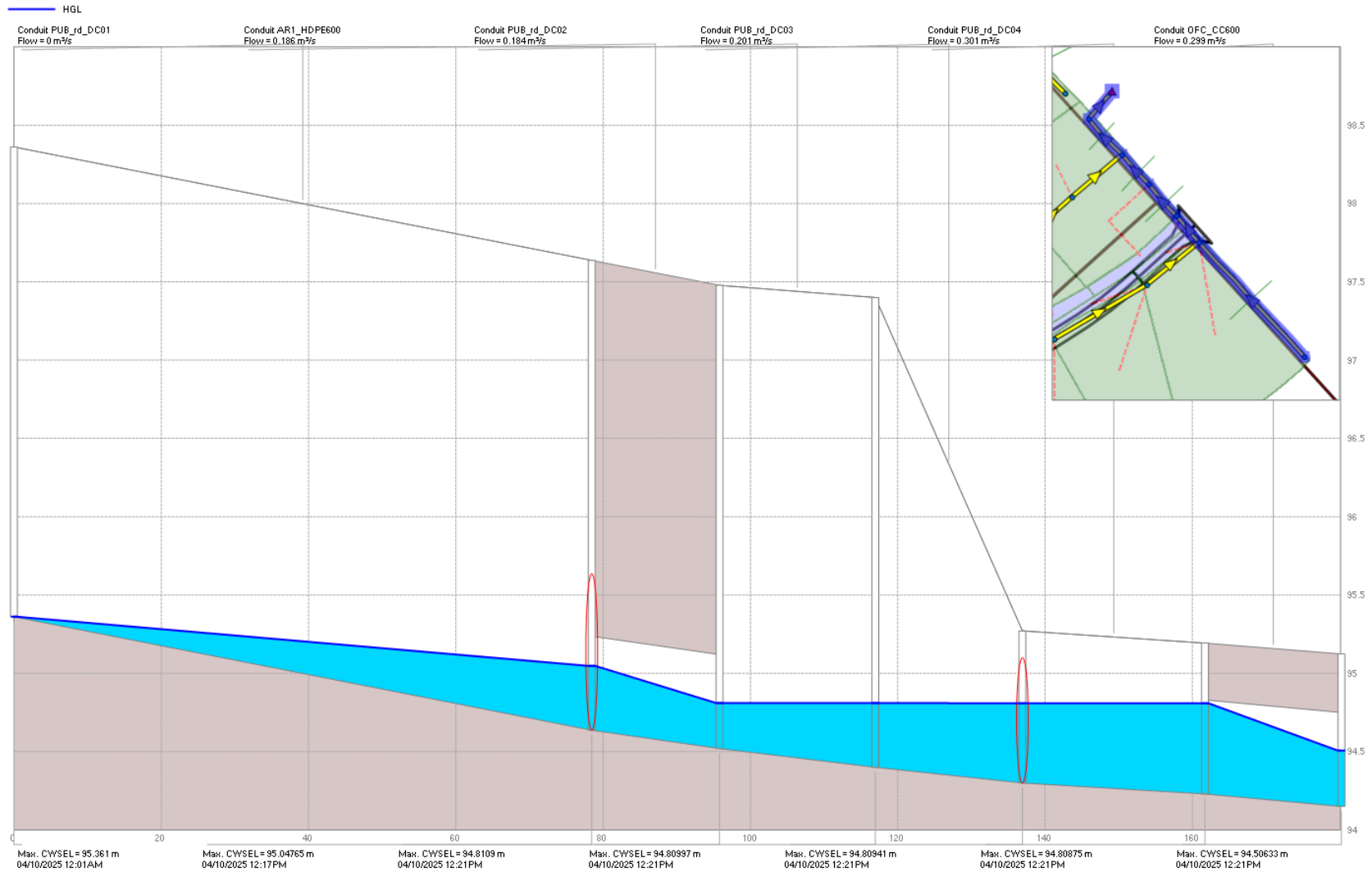
Figure 8: Profile public ditch to outfall C post-development 100y storm event
