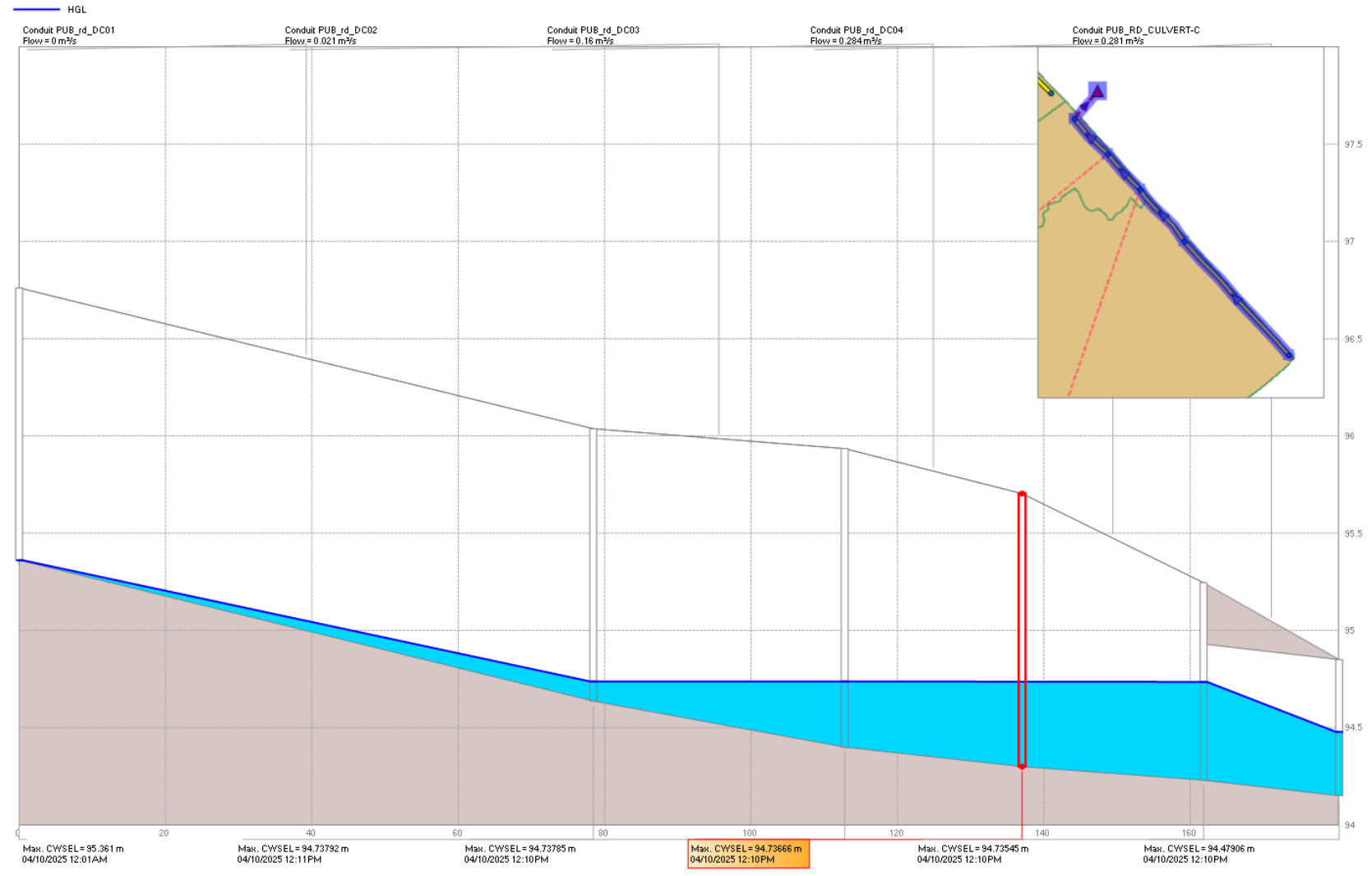
Figure 7: Profile public ditch to outfall C pre-development 100y storm event
