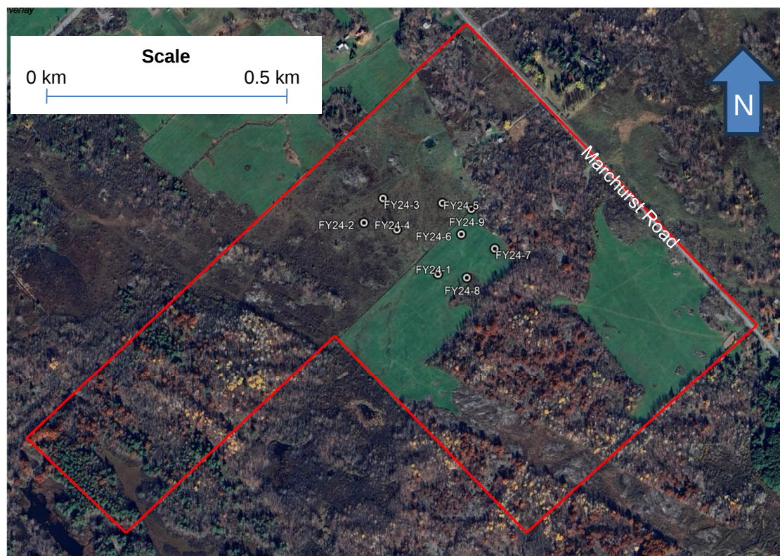
Figure 2-1: Borehole Locations within the South March BESS Project Site
