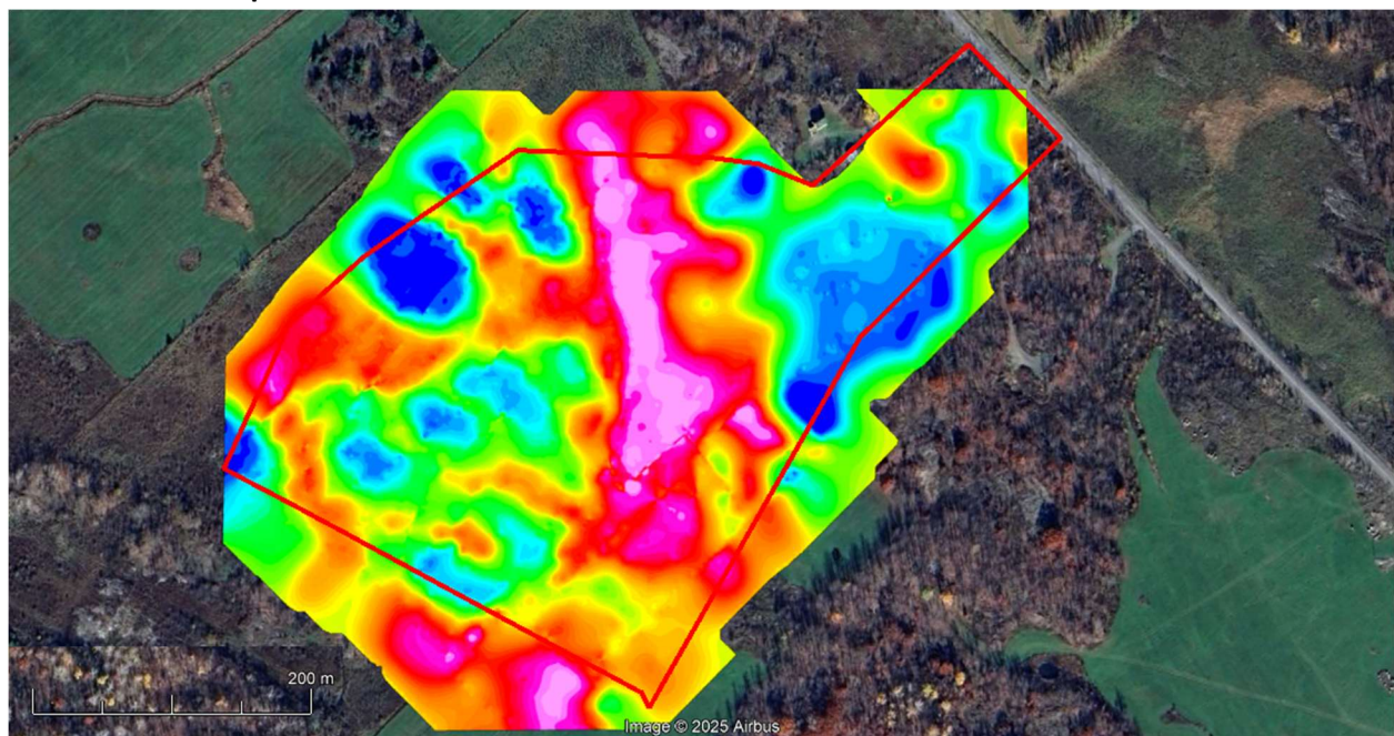
Figure 5: EM-31 Quadrature Ground Conductivity Map
