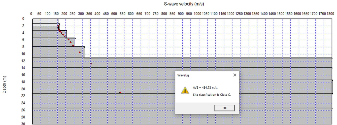
Figure 10: Shear-Wave Model under Line 3
