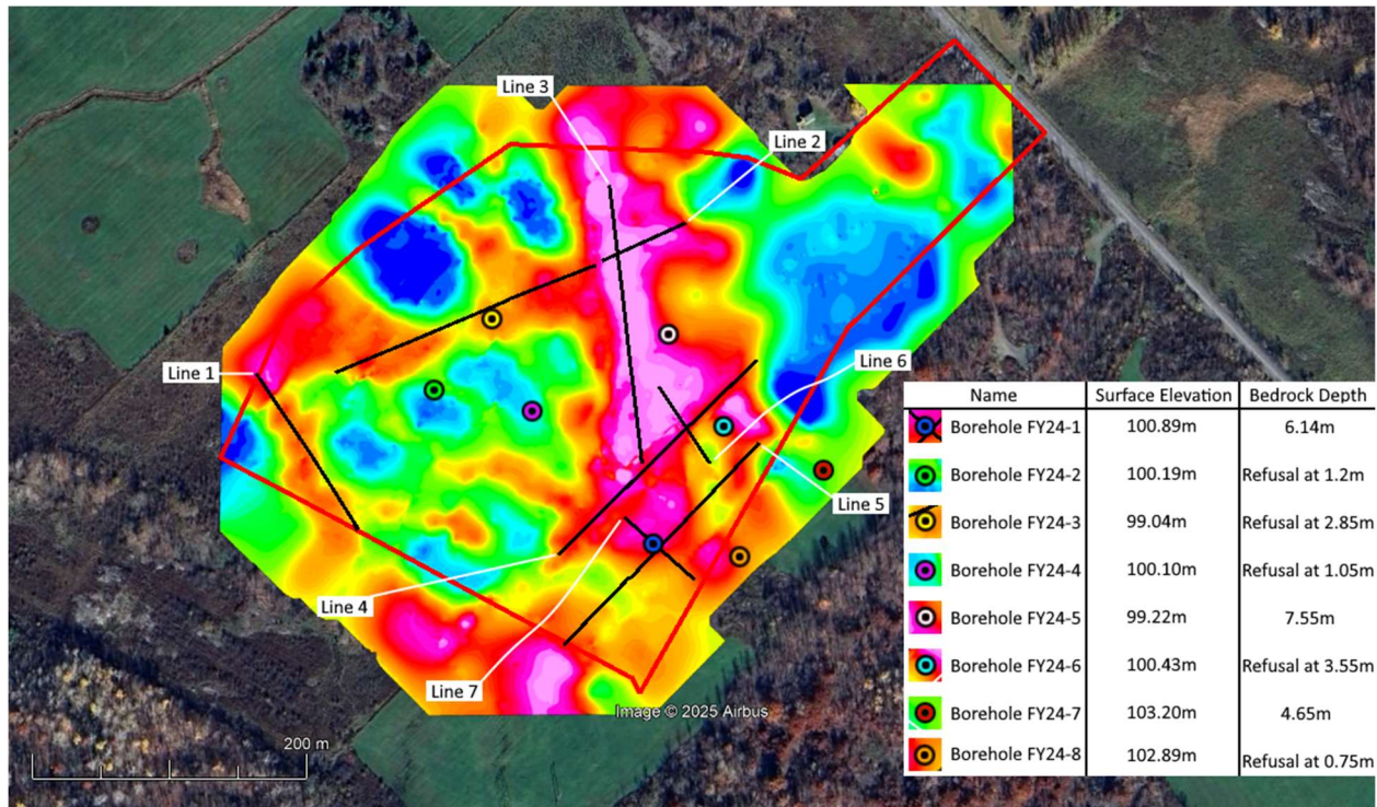
Figure 7: EM-31 Quadrature Phase Ground Conductivity Map with Seismic Line and Borehole Overlay
