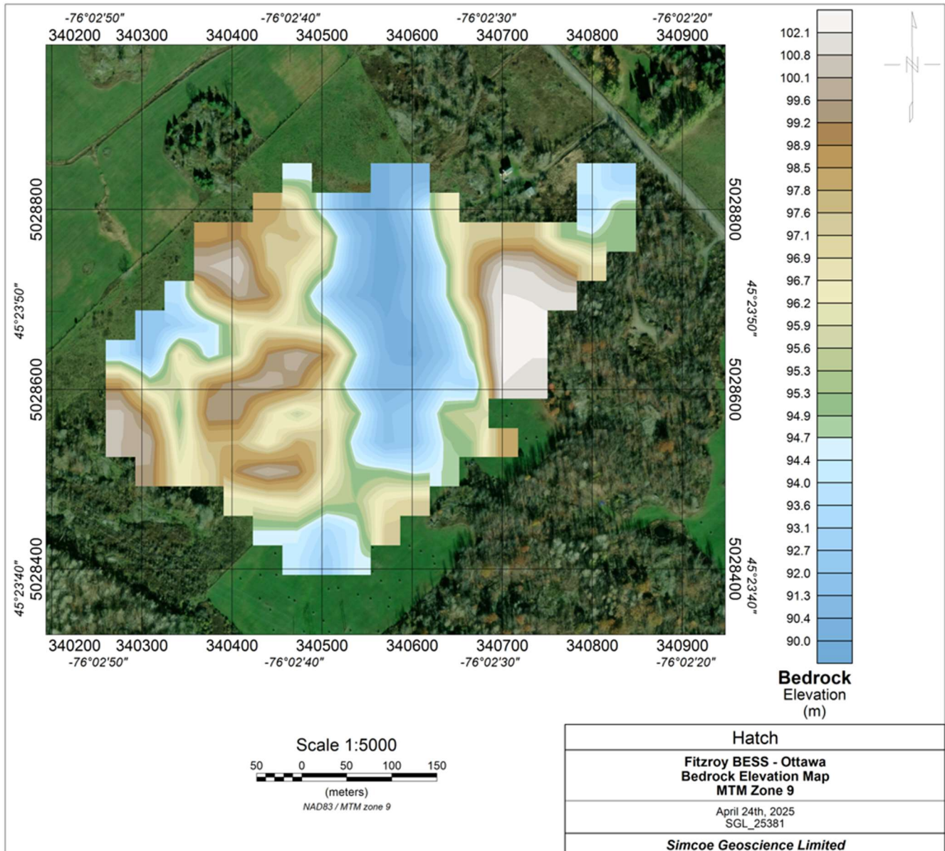
Figure 14: Bedrock Elevation Plot
