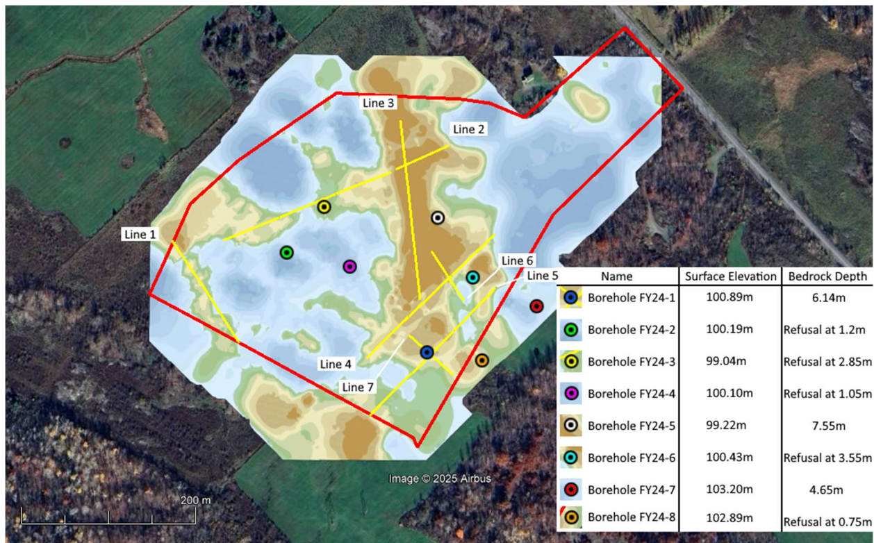
Figure 8: EM-31 In-Phase Magnetic Susceptibility Map with Seismic Line and Borehole Overlay
