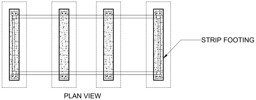
TYPE 3: CONCRETE STRIP FOOTING ACROSS THE LENGTH
