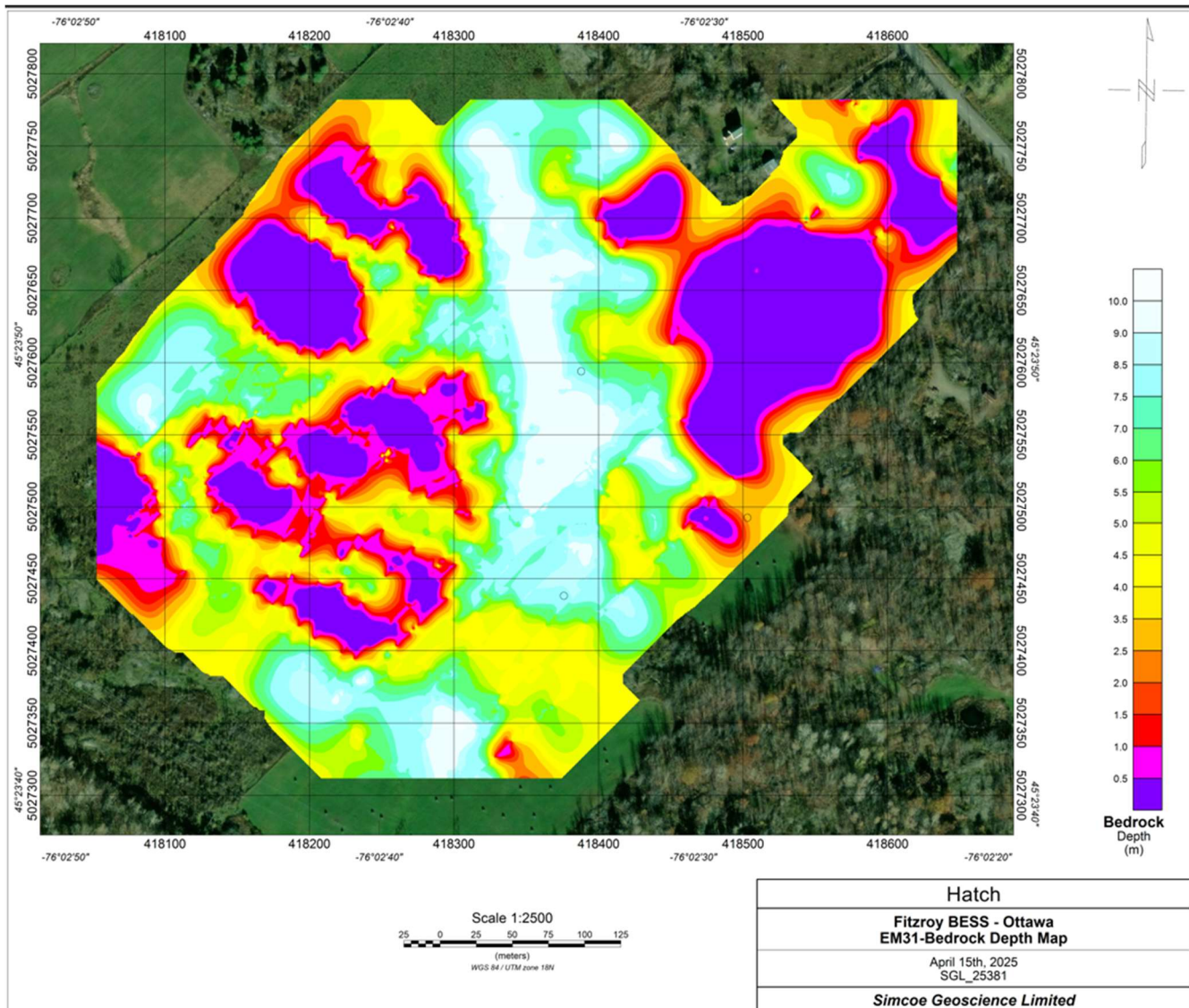
Figure 12: Bedrock Depth Plot
