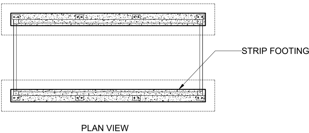
TYPE 4: CONCRETE STRIP FOOTING ALONG THE LENGTH
