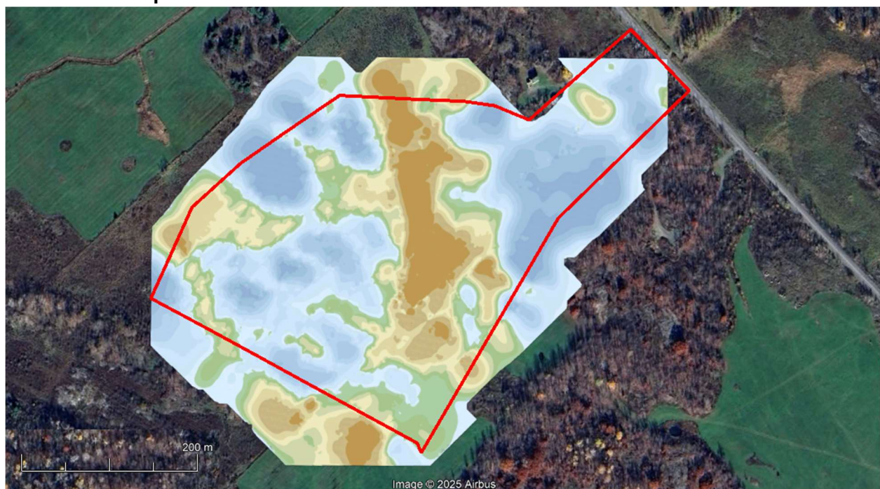
Figure 6: EM-31 In-Phase Magnetic Susceptibility Map
