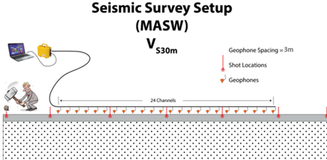
Figure 3: Seismic 3-meter Spacing Field Setup, Geophones (orange), Shot Locations (red)
