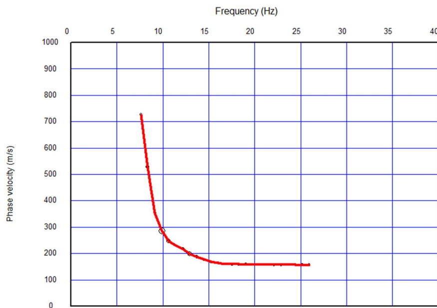
Figure 9: Combined Active & Passive Dispersion Curve for the MASW test
