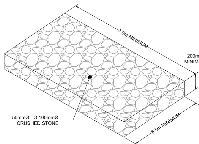
MUD MAT DETAIL
