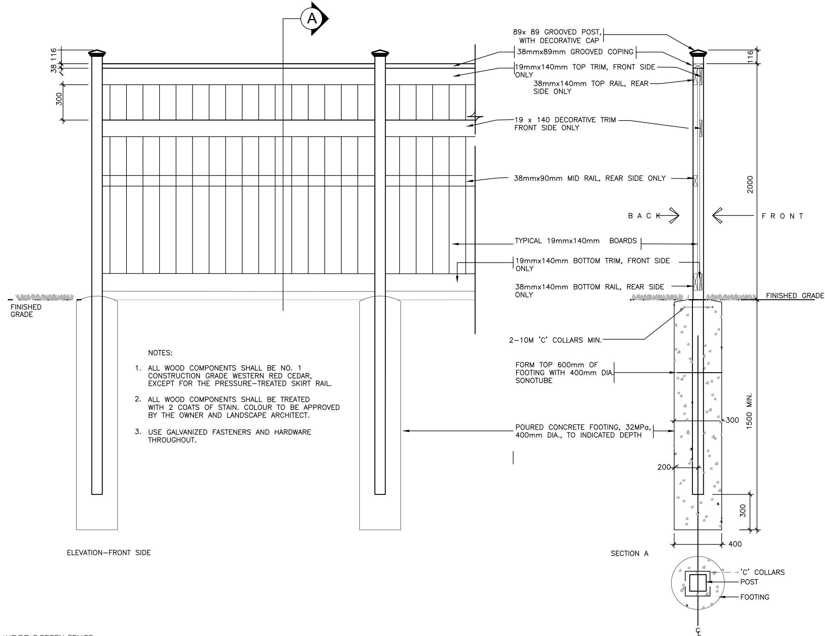
3 WOOD SCREEN FENCE Scale: 1:20
