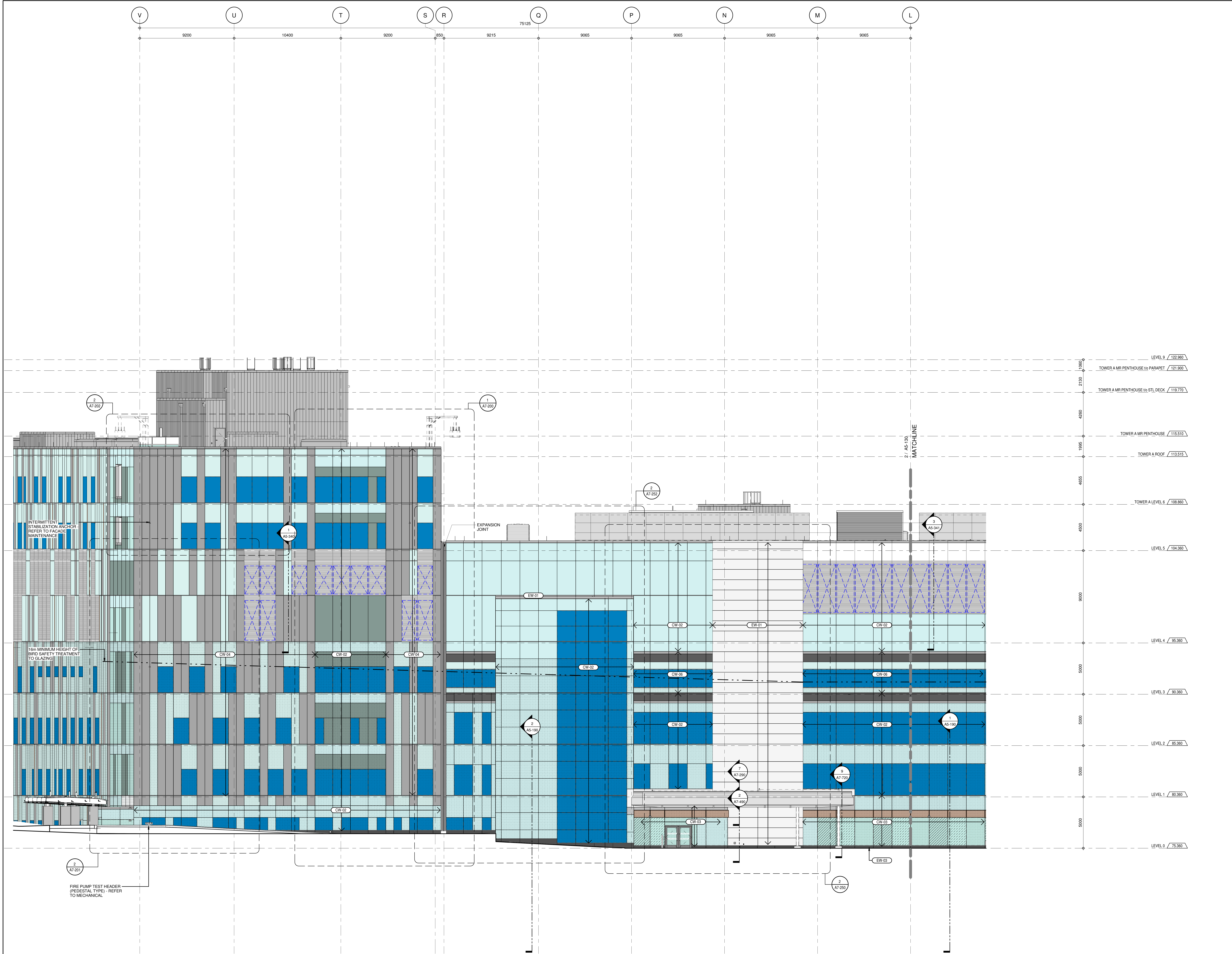
ELEVATION - SOUTH TRUE ELEVATION TOWER A AND PODIUM
