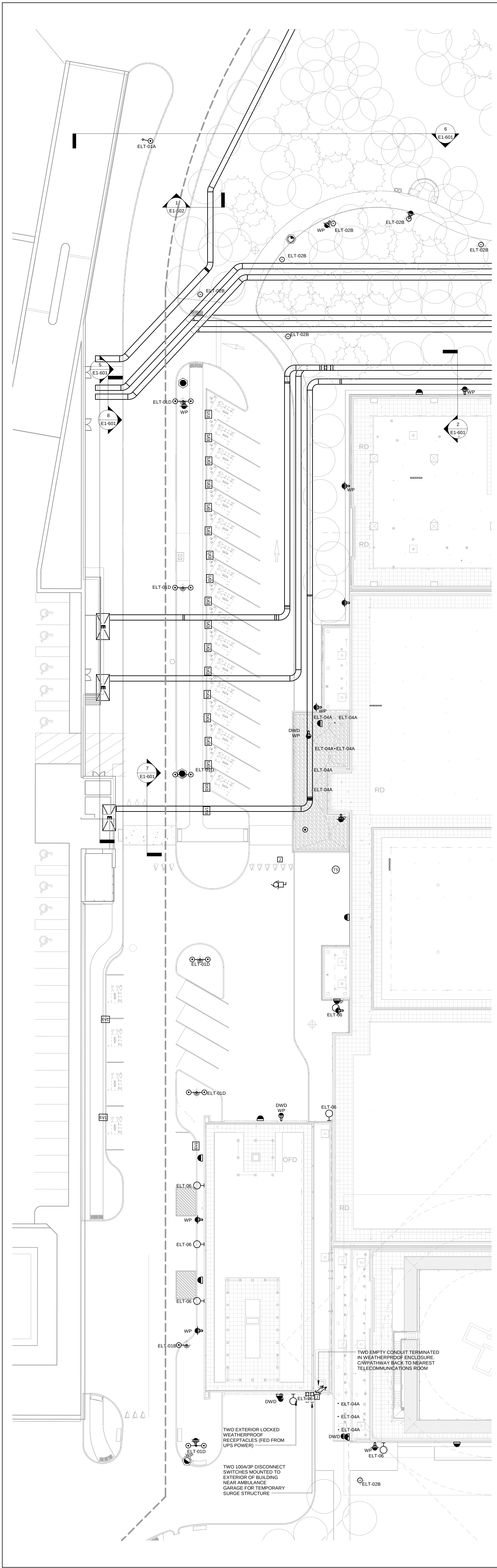
3 ELECTRICAL - ZONE 5A LEVEL 0 - EMERGENCY SERVICES PARKING (SOUTH) E1-101.1 1: 250
