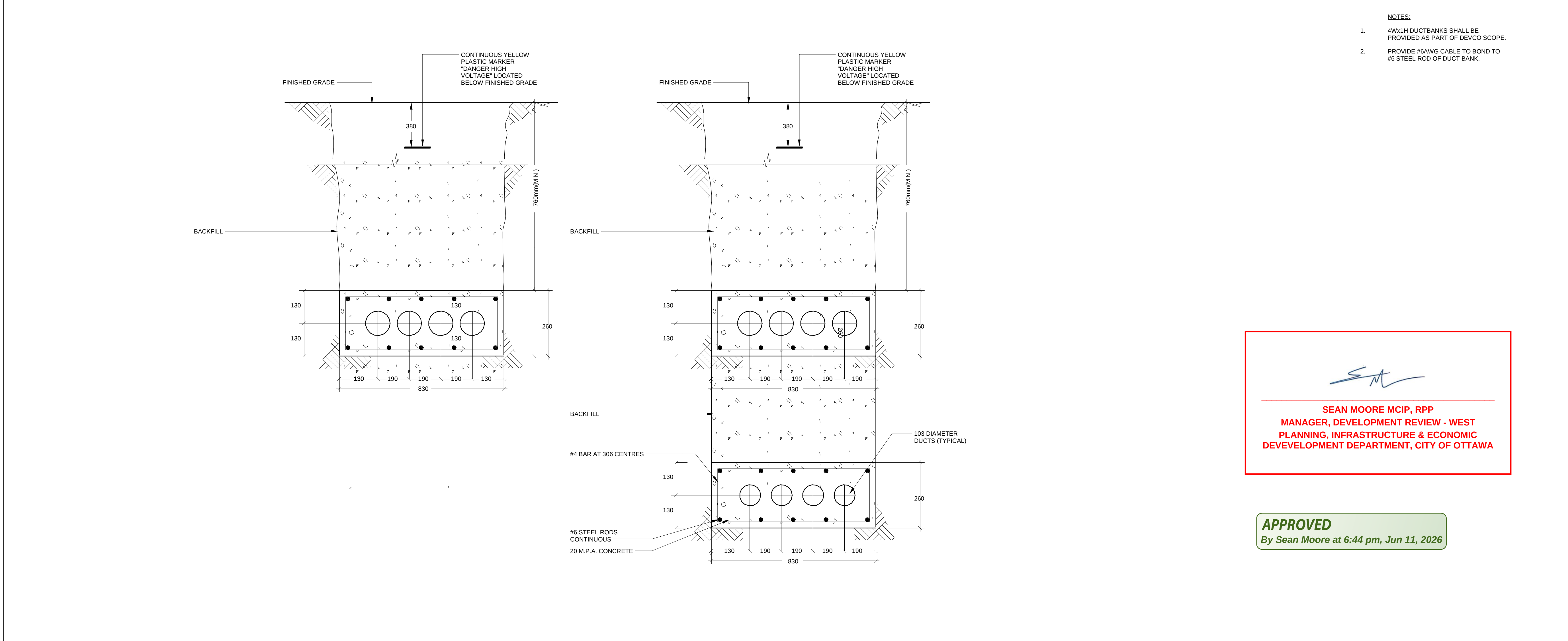
2 EMERGENCY POWER DUCT BANK DETAIL FROM MANHOLE E1-601 N.T.S.
