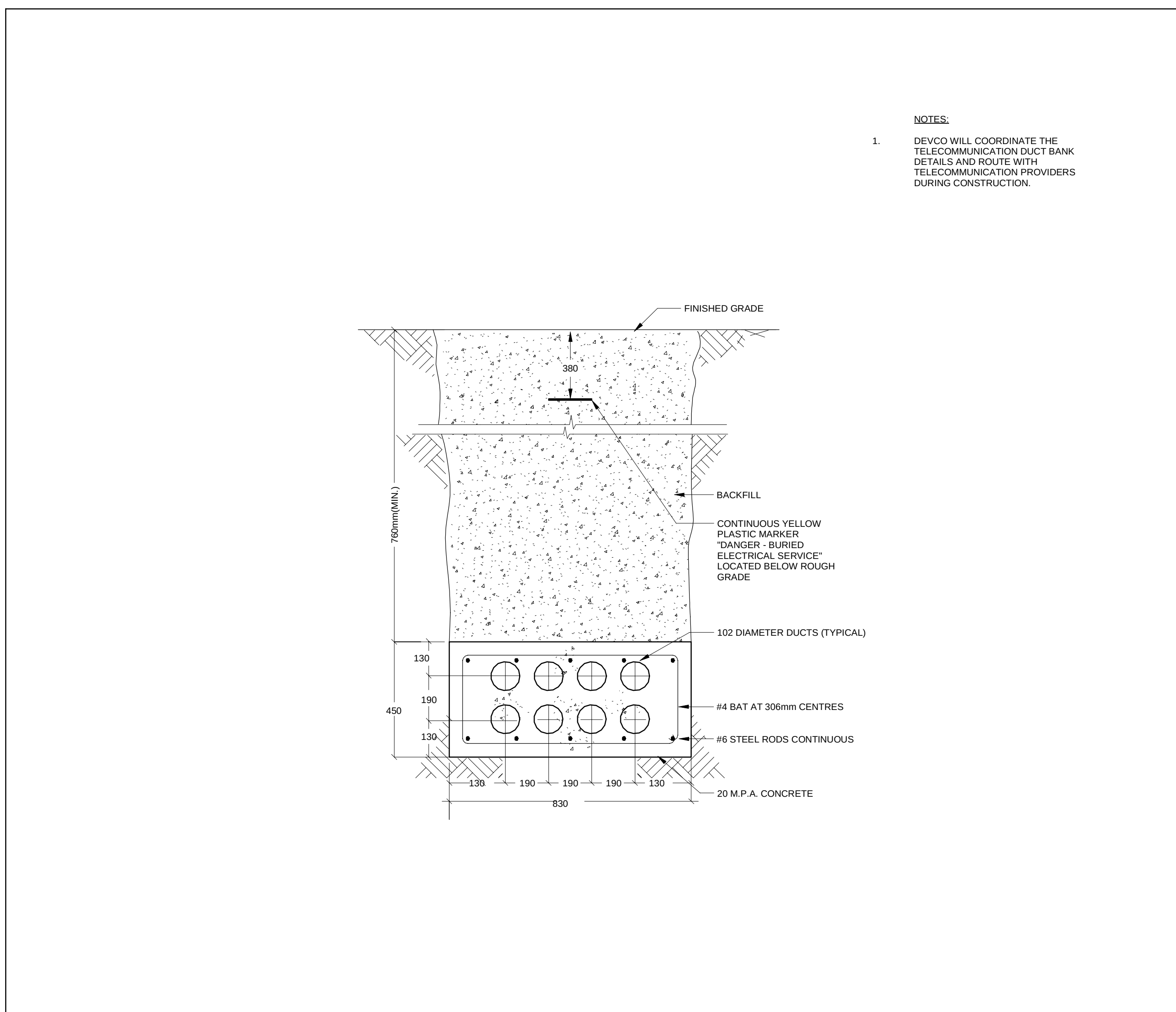
4 TELECOMM DUCT BANK - ENTRANCE FACILITY SOUTH E1-601 N.T.S.
