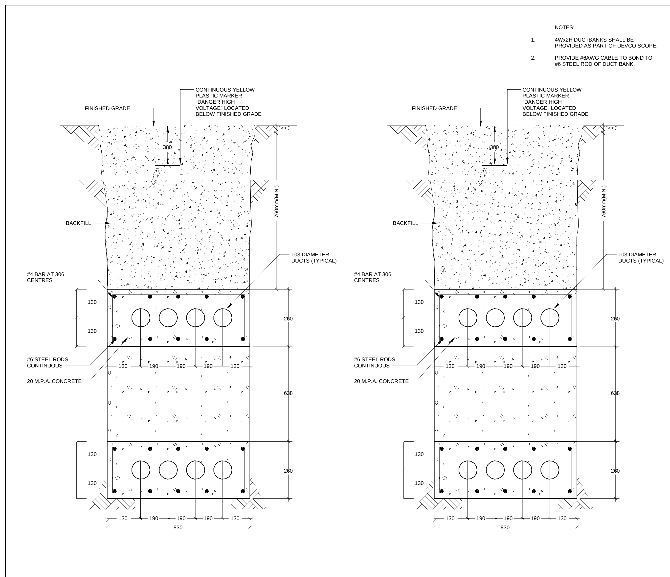
8 NORMAL POWER DUCT BANK DETAIL TO MANHOLE (FROM CUP) E1-601 N.T.S.
