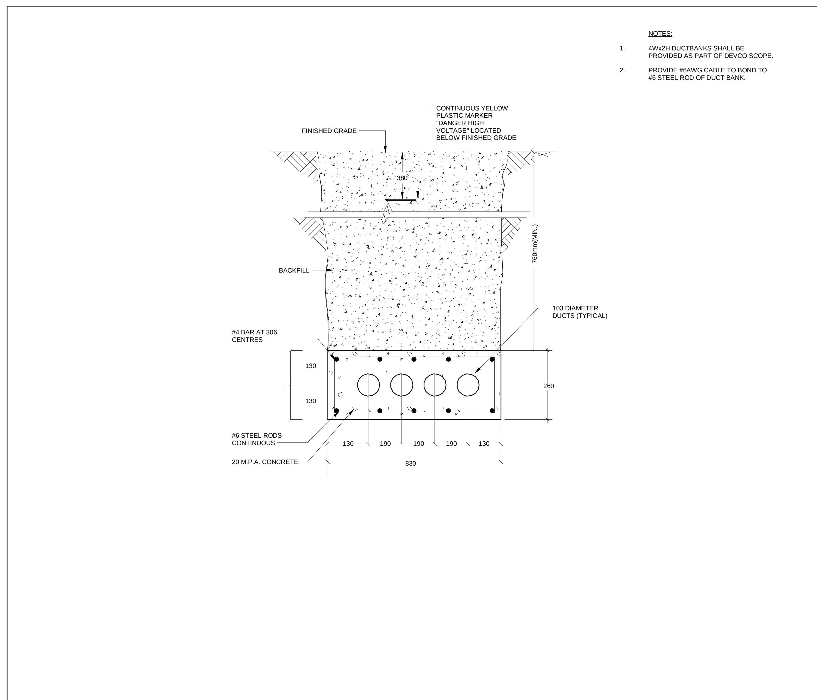
7 EMERGENCY POWER DUCT BANK DETAIL TO MANHOLE (FROM CUP TYPICAL OF THREE) E1-601 N.T.S.
