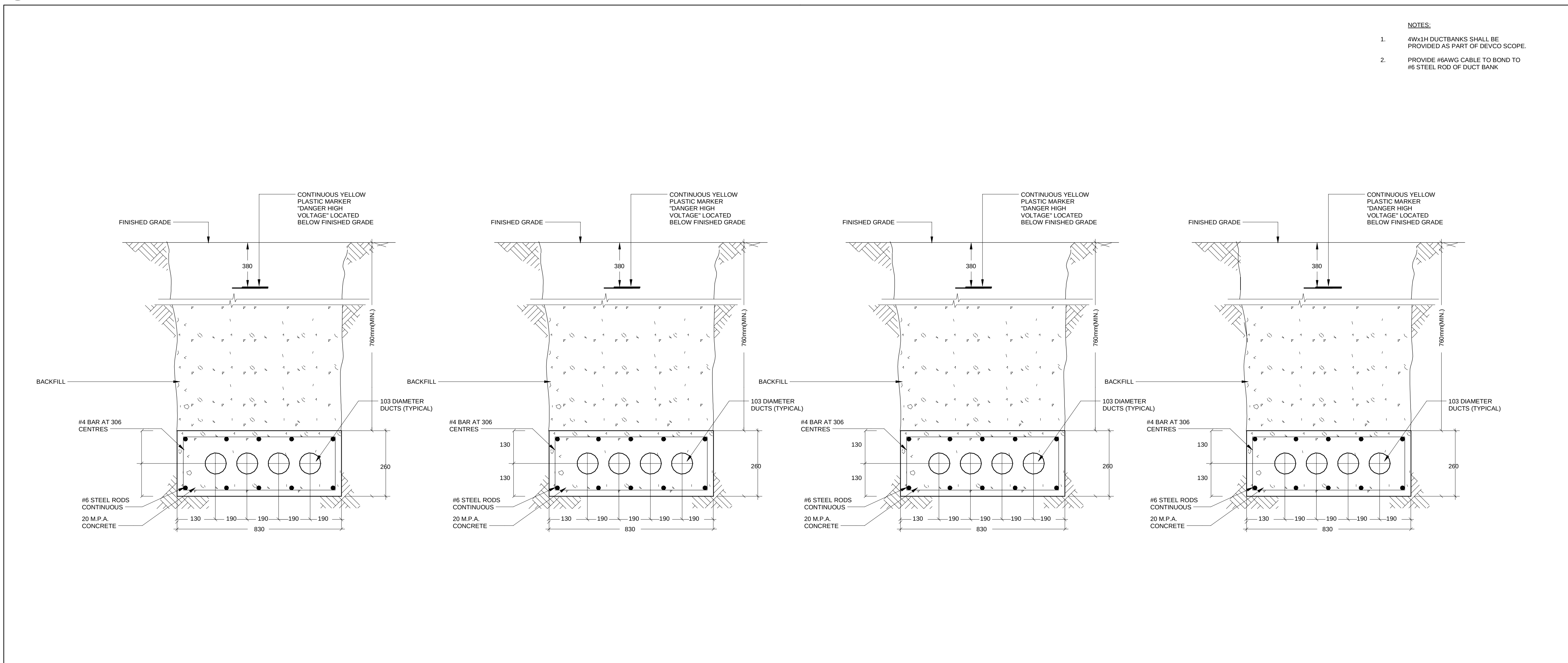
1 NORMAL POWER DUCT BANK DETAIL FROM MANHOLE E1-601 N.T.S.
