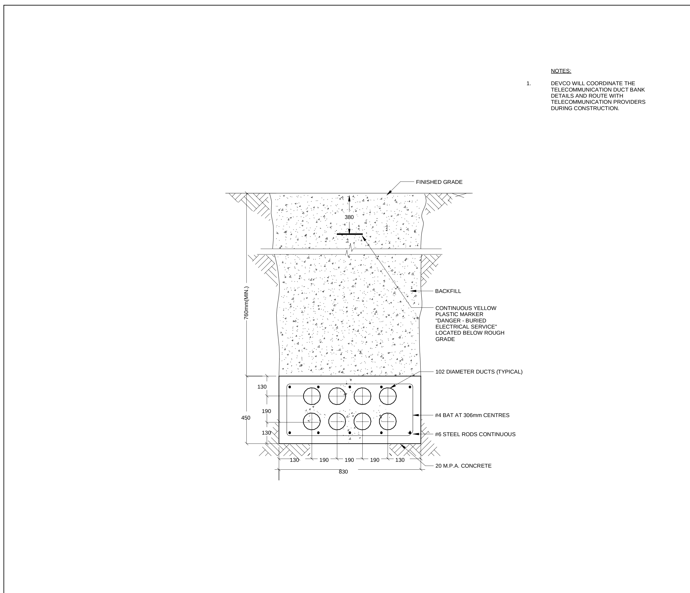
3 TELECOMM DUCT BANK - ENTRANCE FACILITY NORTH E1-601 N.T.S.
