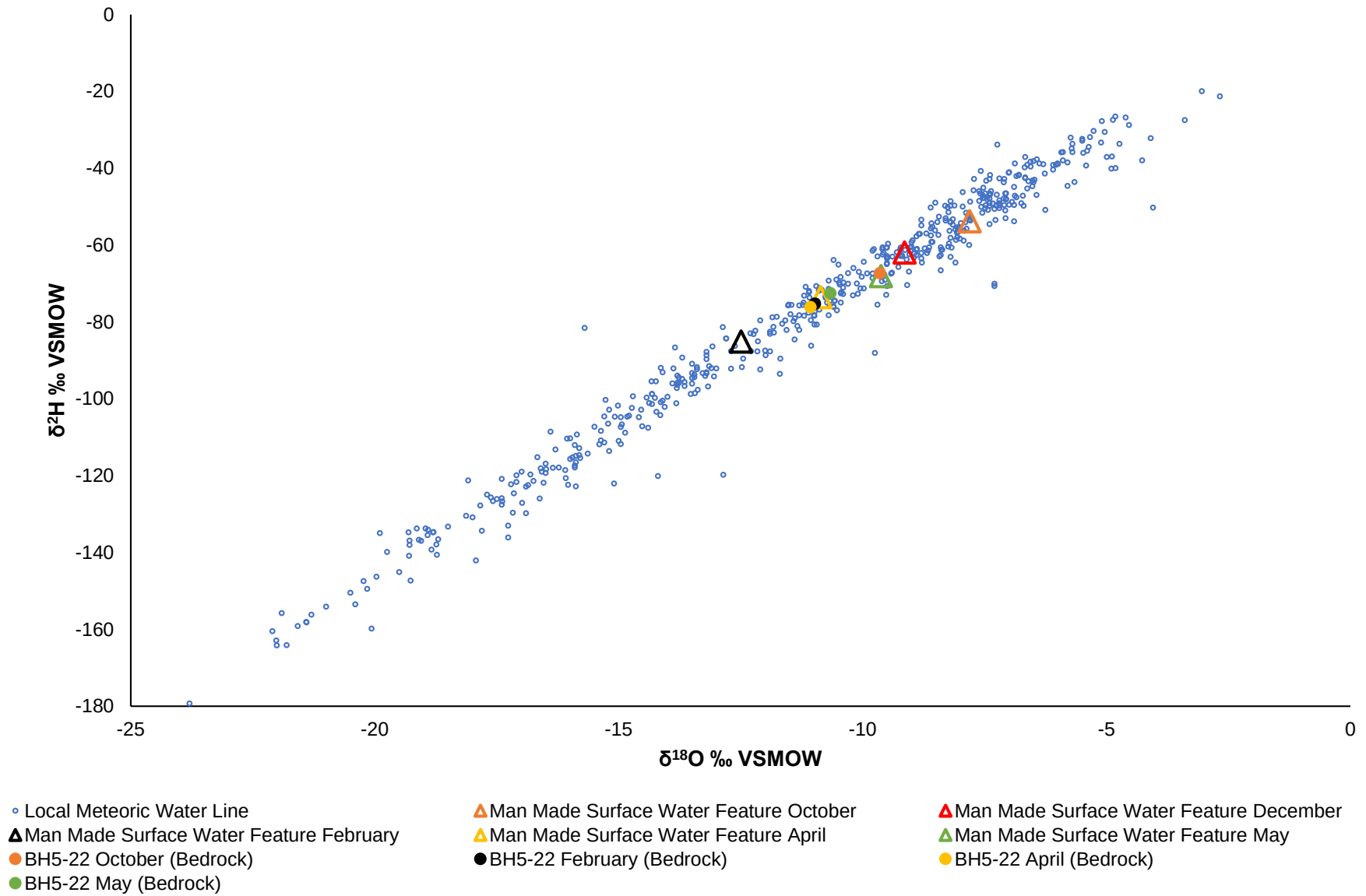
Figure 15: BH5-22 \delta^2\text{H}/\delta^{18}\text{O} Results
