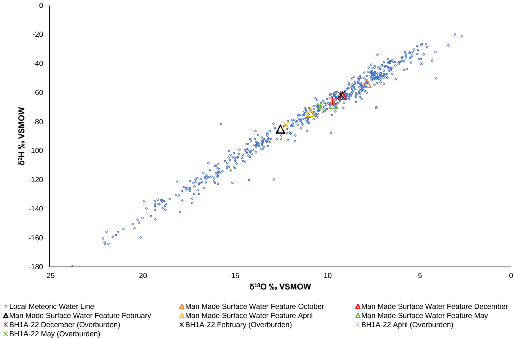
Figure 16: BH1A-22 \delta^2\text{H}/\delta^{18}\text{O} Results
