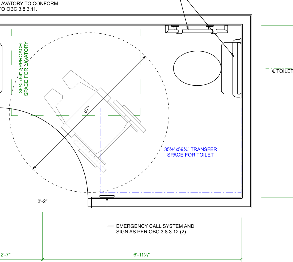
UNIVERSAL WASHROOM DETAIL SCALE: 1/2" = 1'-0"
